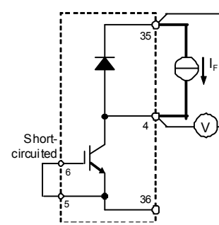
Brake IGBT
