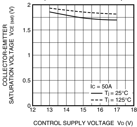
COLLECTOR-EMITTER SATURATION VOLTAGE (VS. V_D ) CHARACTERISTICS (INVERTER PART - TYPICAL)
