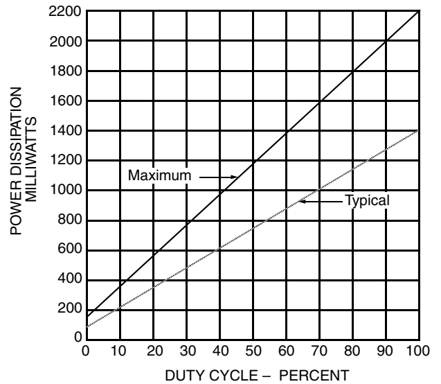
FIGURE 6 – POWER DISSIPATION VS. DUTY CYCLE
