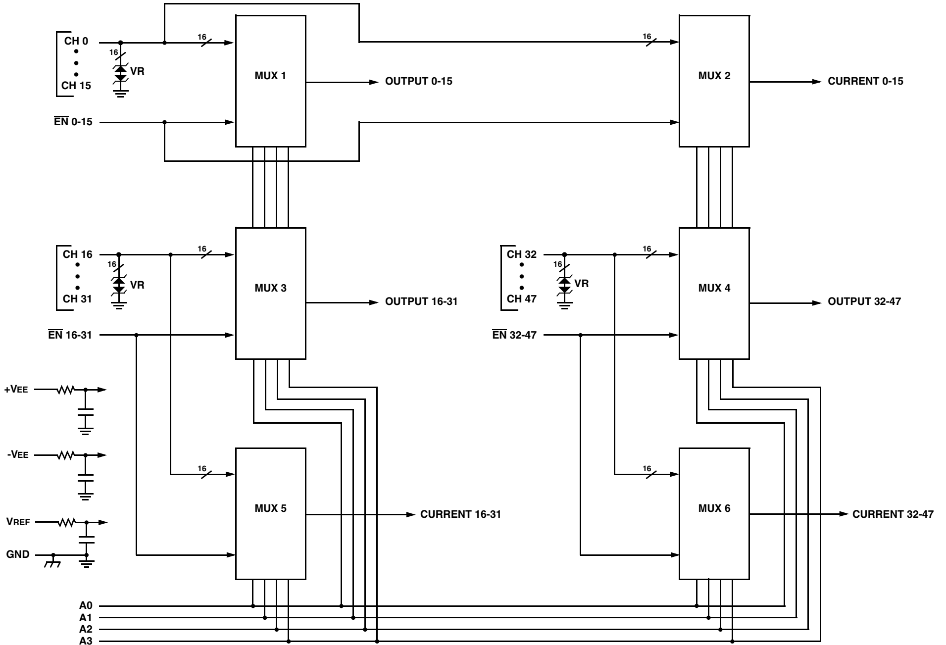
ACT8512 48-CHANNEL ANALOG MUX BLOCK DIAGRAM
