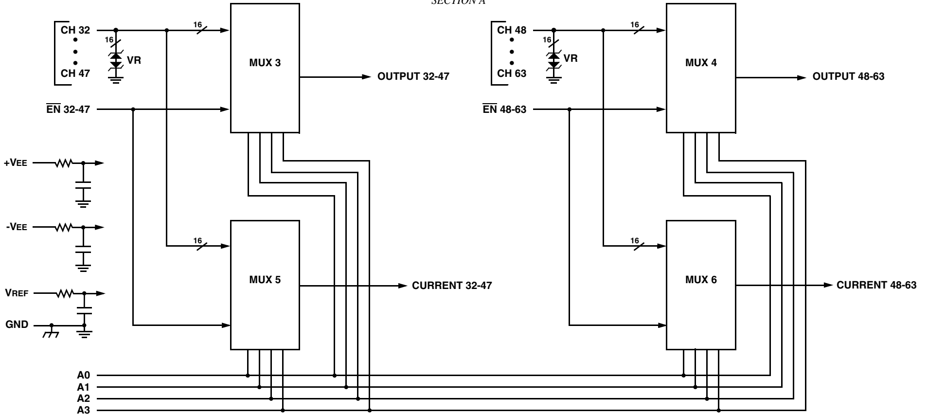
ACT8500 64-CHANNEL ANALOG MUX BLOCK DIAGRAM
