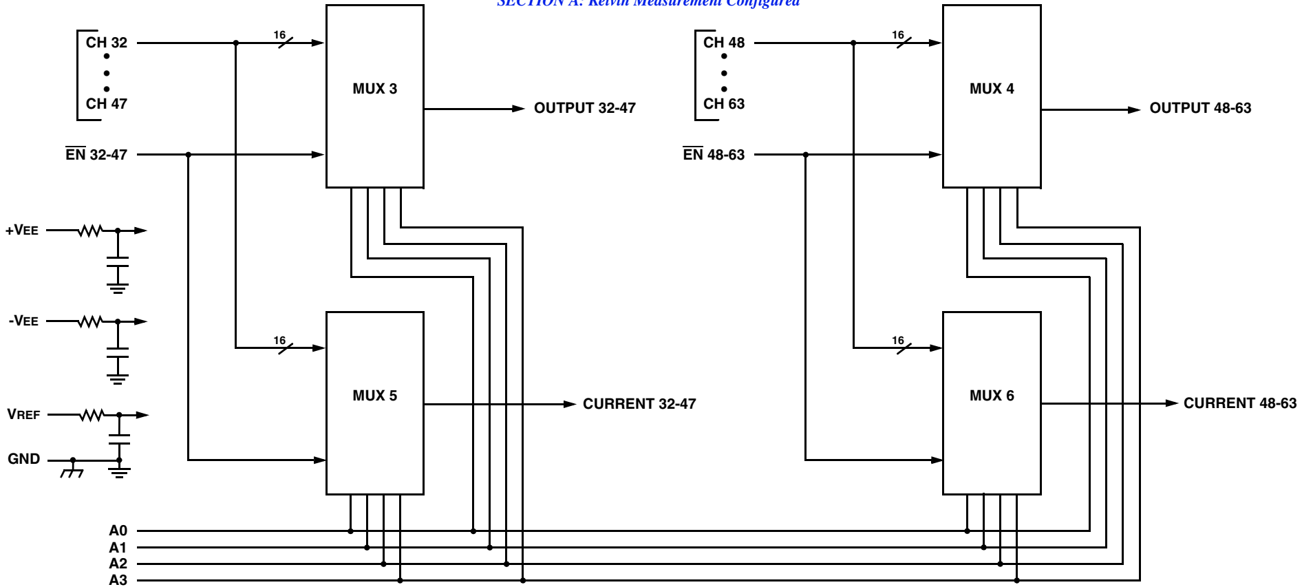
MUX8507 64-CHANNEL ANALOG MUX BLOCK DIAGRAM
