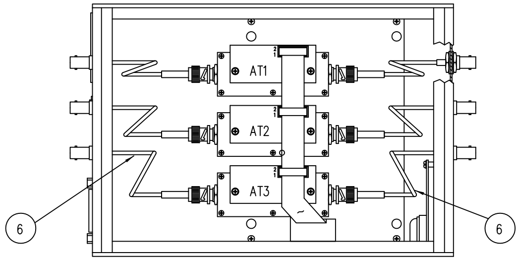
-T CONFIGURATIONS
