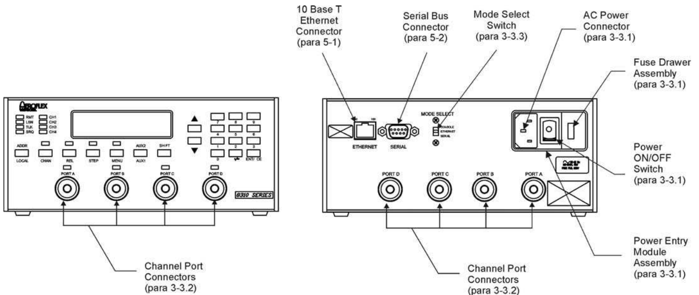
Figure 2. Rear Panel Controls & Connectors
