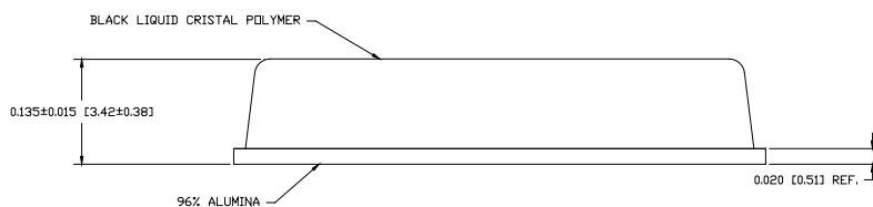
SMT680 PACKAGE OUTLINE
