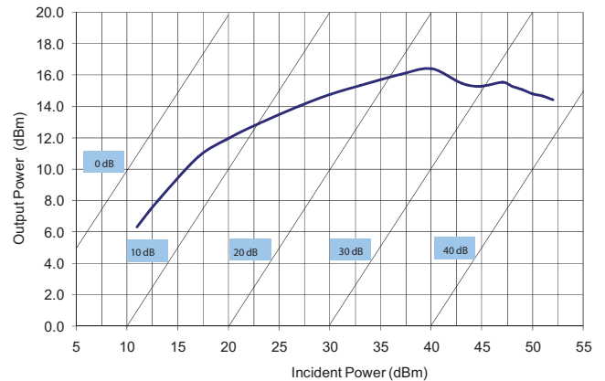
Flat Leakage Output Power vs. Input Power, Pulse width = 10 \mu\text{s} , Duty Cycle = 1%, f = 2 \text{ GHz}
