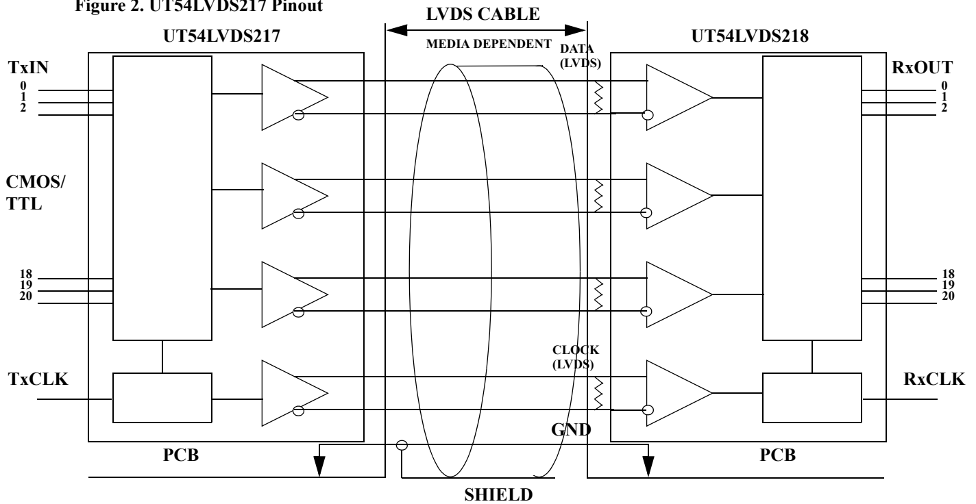
Figure 3. UT54LVDS217 Typical Application
