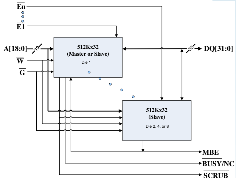
Figure 1. Block Diagram
