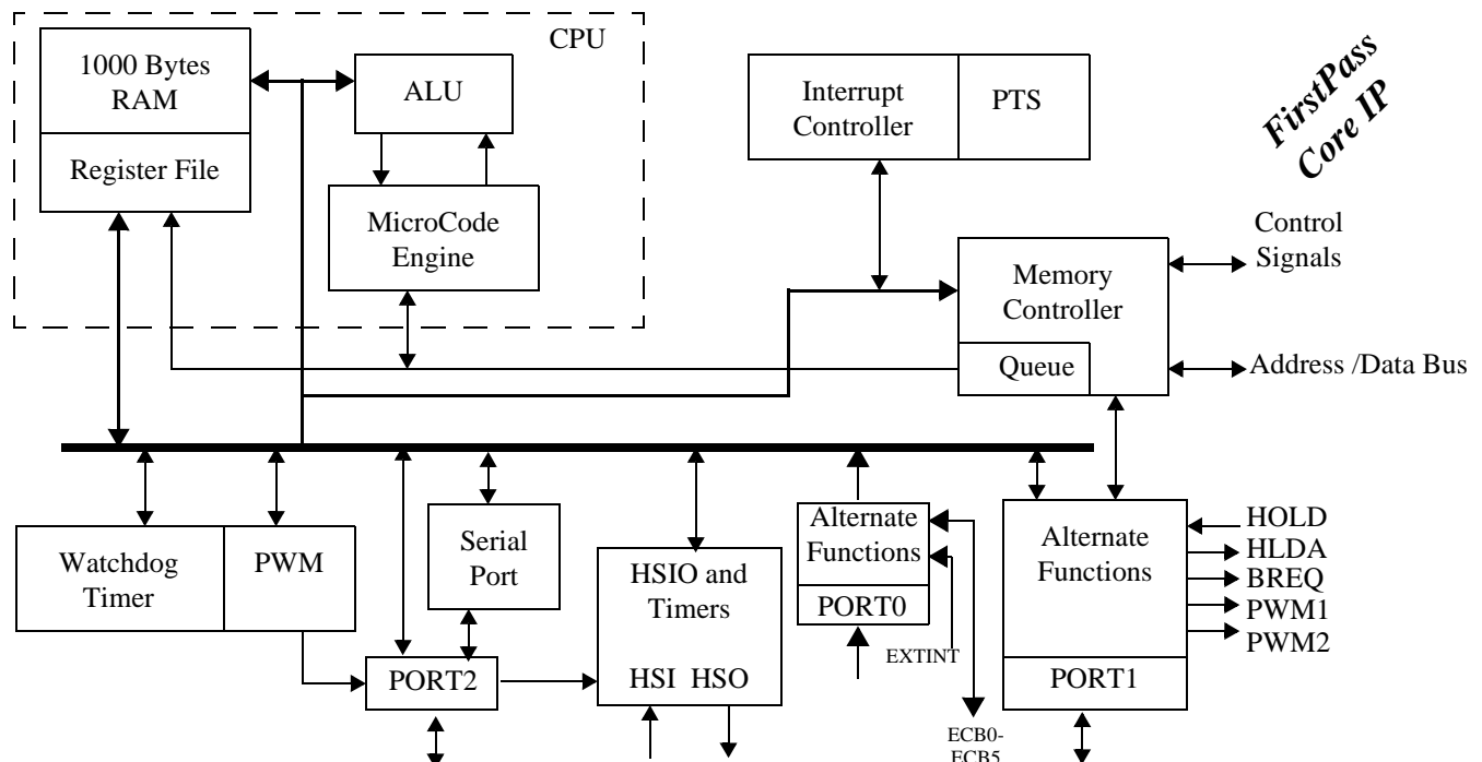
Figure 1. UT80CRH196KDS Microcontroller
