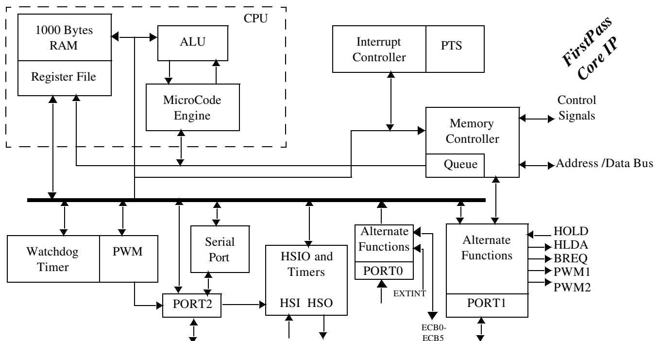
Figure 1. UT80C196KDS Microcontroller
