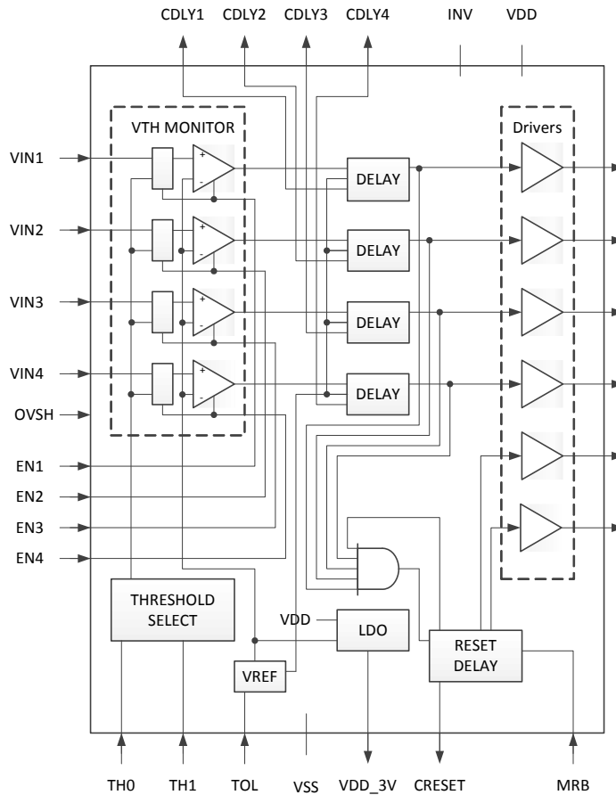
Figure 1. UT04VS50P Block Diagram
