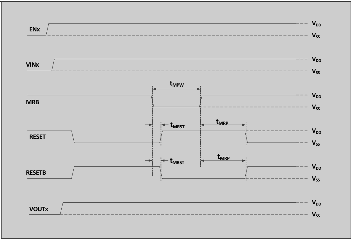
Figure 5. MRB Timing Diagram
