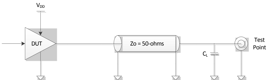
Figure 3: Test Circuit Load used for AC timing
