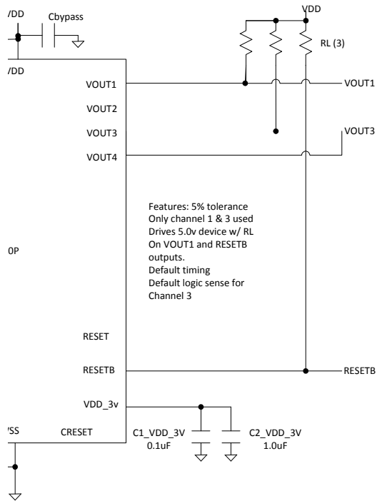
Figure 7. Application example of basic connection
