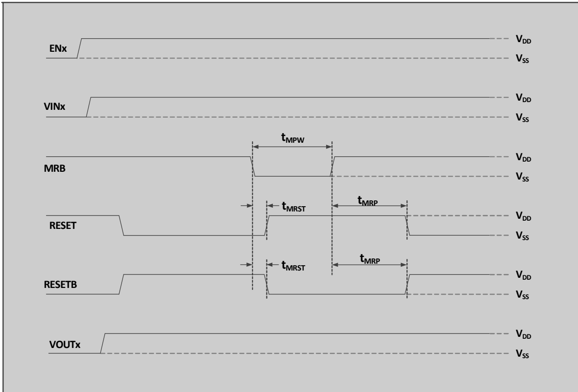
Figure 6. VINx Timing Diagram
