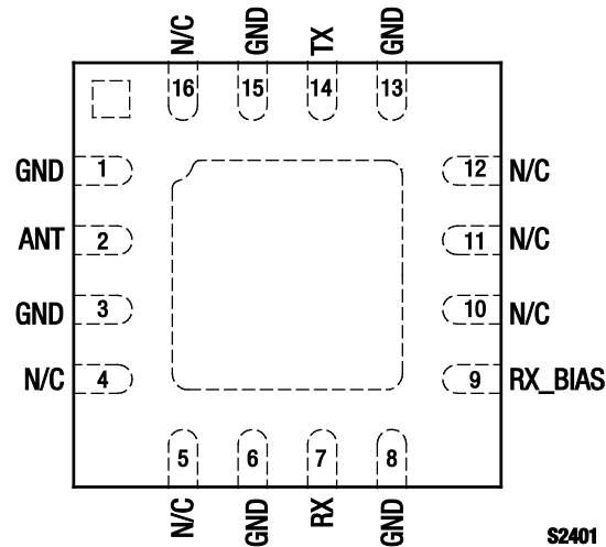
Figure 2. SKY12208-306LF Pinout – 16-Pin QFN (Top View)
