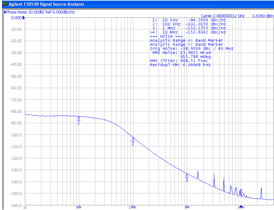
Figure 16. Closed-Loop Phase Noise Performance For RFour = 2.8 GHz (FSTEP = 1600 kHz, VCO_Div = 1, FCOMP = 1.6 MHz)
