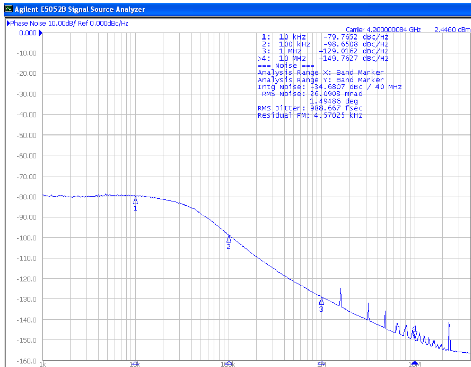
Figure 17. Closed-Loop Phase Noise Performance For RFour = 4.2 GHz (FSTEP = 1600 kHz, VCO_Div = 1, FCOMP = 1.6 MHz)
