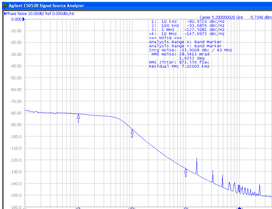
Figure 18. Closed-Loop Phase Noise Performance For RFour = 5.2 GHz (FSTEP = 1600 kHz, VCO_Div = 1, FCOMP = 1.6 MHz)
