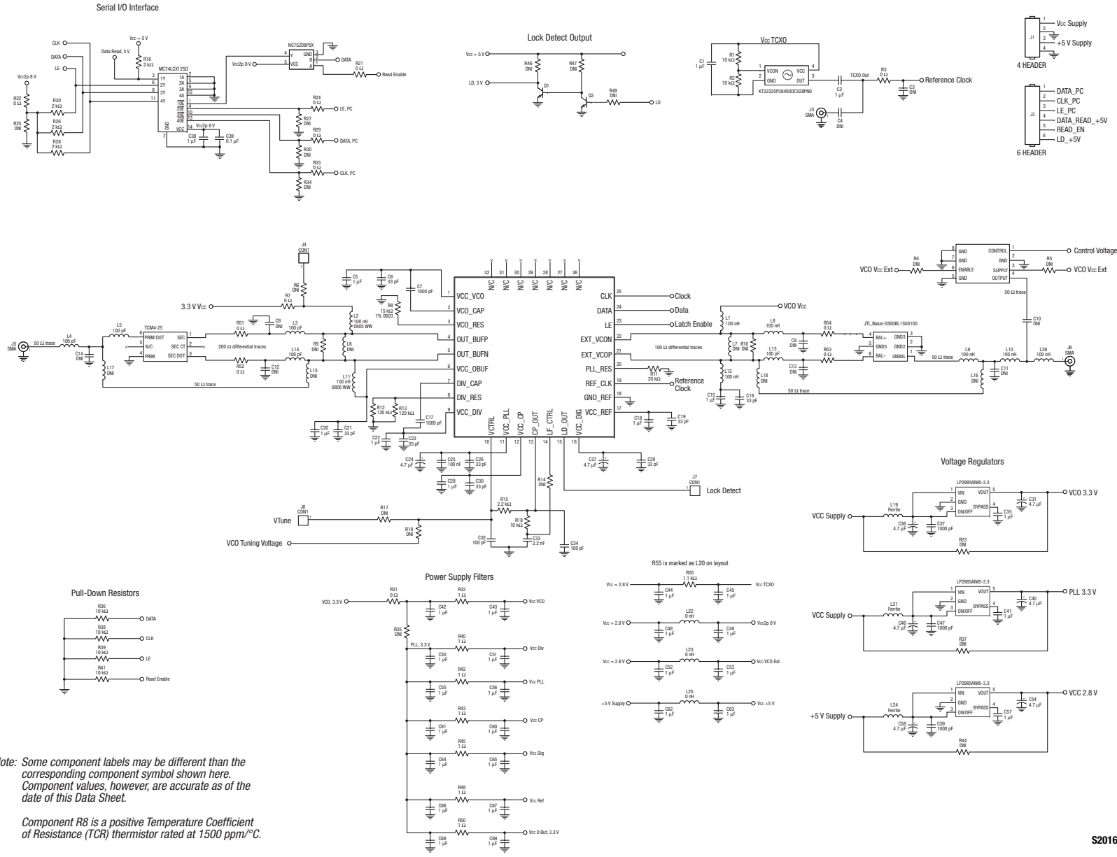
Figure 22. SKY73134-11 Evaluation Board Schematic
