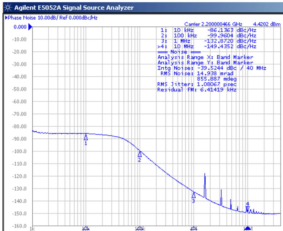
Figure 15. Closed-Loop Phase Noise Performance For RFour = 2.2 GHz (FSTEP = 800 kHz, VCO_Div = 2, FCOMP = 1.6 MHz)
