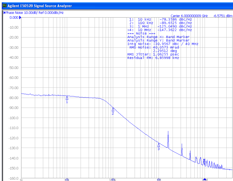
Figure 19. Closed-Loop Phase Noise Performance For RFour = 6.0 GHz (FSTEP = 1600 kHz, VCO_Div = 1, FCOMP = 1.6 MHz)
