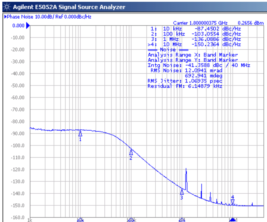
Figure 14. Closed-Loop Phase Noise Performance For RFour = 1.8 GHz (FSTEP = 400 kHz, VCO_Div = 3, FCOMP = 1.2 MHz)
