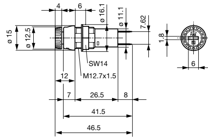
Variants Fingergrrip 3101.0015 and 3101.0215
