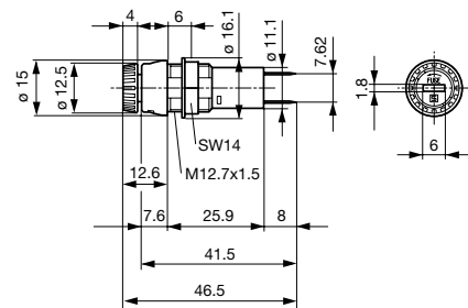
Variants Fingergrrip 3101.0115 and 3101.0315
