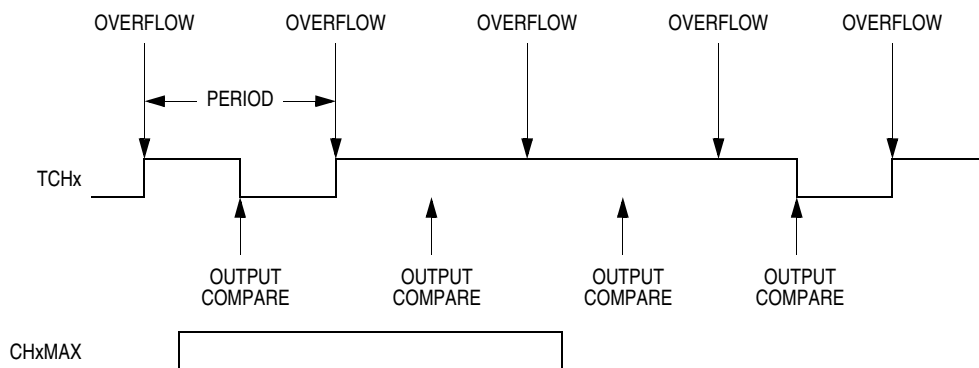
Figure 18-9. CHxMAX Latency
