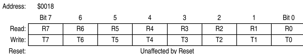
Figure 14-16. SCI Data Register (SCDR)
