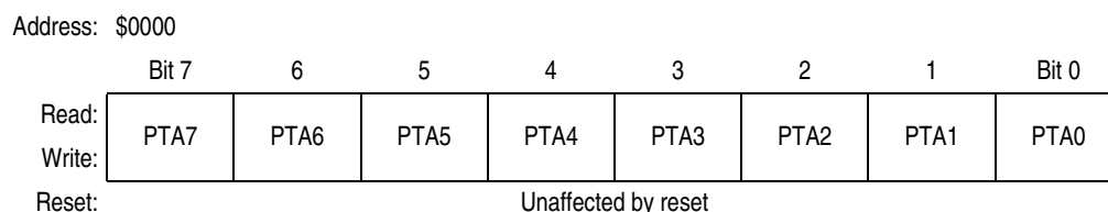
Figure 13-2. Port A Data Register (PTA)
