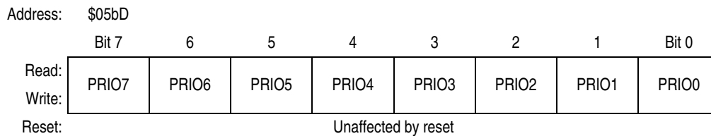
Figure 11-14. Transmit Buffer Priority Register (TBPR)
