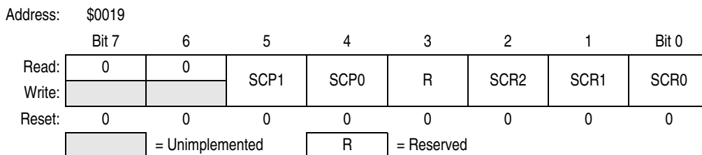
Figure 14-17. SCI Baud Rate Register (SCBR)
