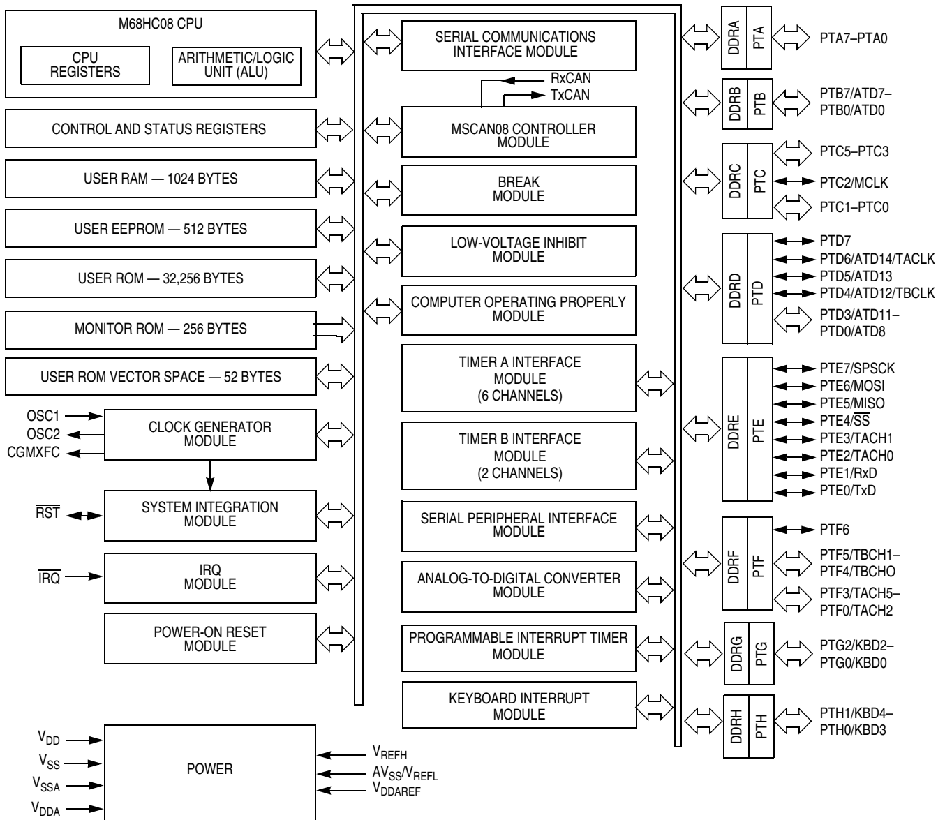
Figure 1-1. MC68HC08AZ32A MCU Block Diagram
