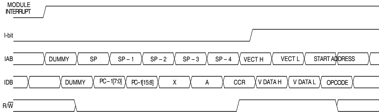
Figure 8-7. Interrupt Entry
