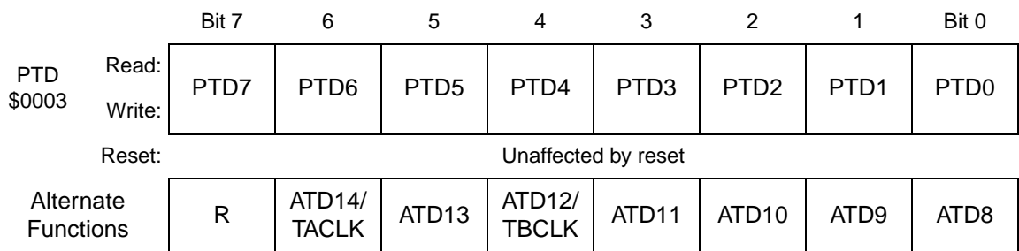
Figure 20-10. Port D Data Register (PTD)
