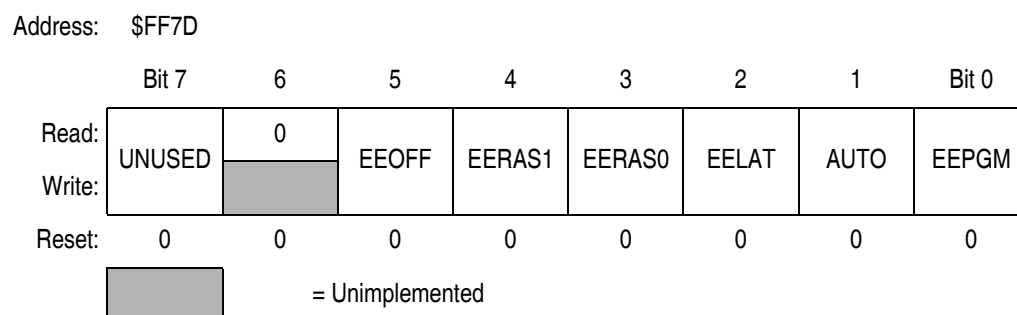
Figure 6-2. EEPROM-2 Control Register (EE2CR)
