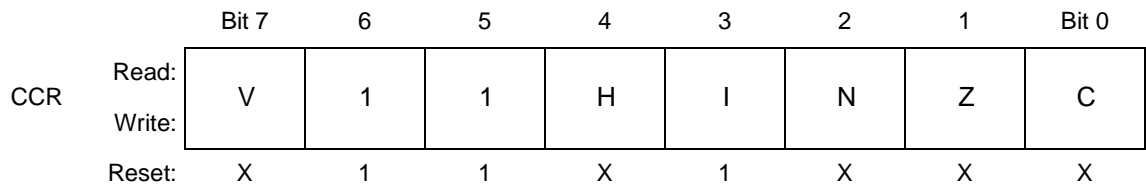
Figure 7-6. Condition Code Register (CCR)
