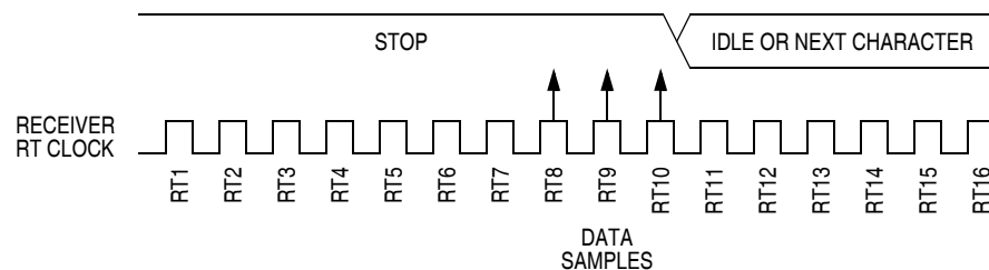
Figure 16-10. Fast Data
