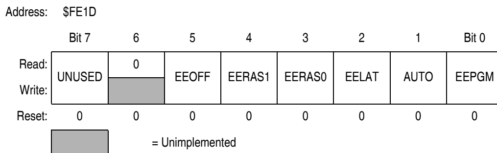
Figure 5-2. EEPROM-1 Control Register (EE1CR)
