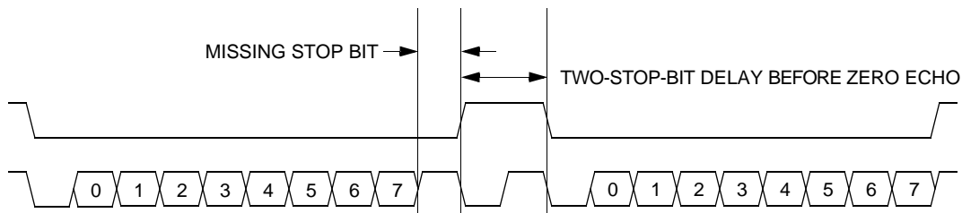
Figure 12-5. Break Transaction
