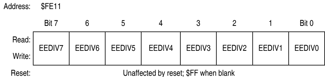
Figure 5-8. EEPROM-1 Divider Non-Volatile Register Low (EE1DIVLNVR)
