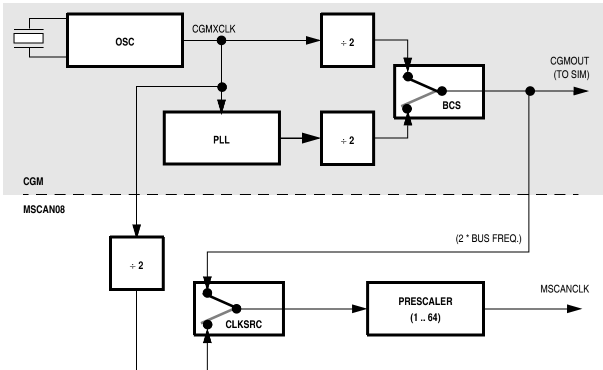
Figure 21-7. Clocking Scheme
