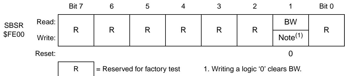
Figure 8-15. SIM Break Status Register (SBSR)
