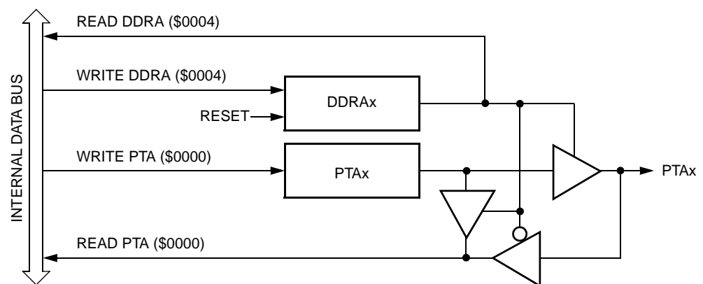
Figure 20-3. Port A I/O Circuit
