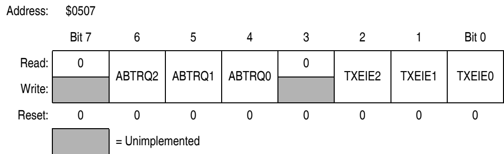
Figure 21-22. Transmitter Control Register (CTCR)
