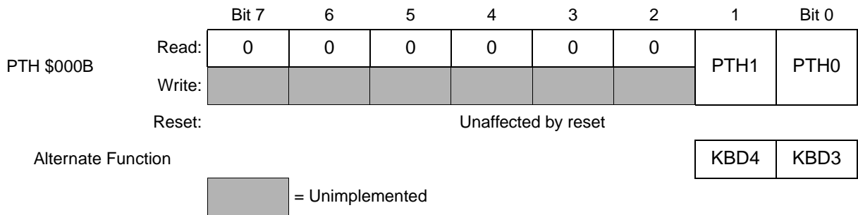
Figure 20-22. Port H Data Register (PTH)
