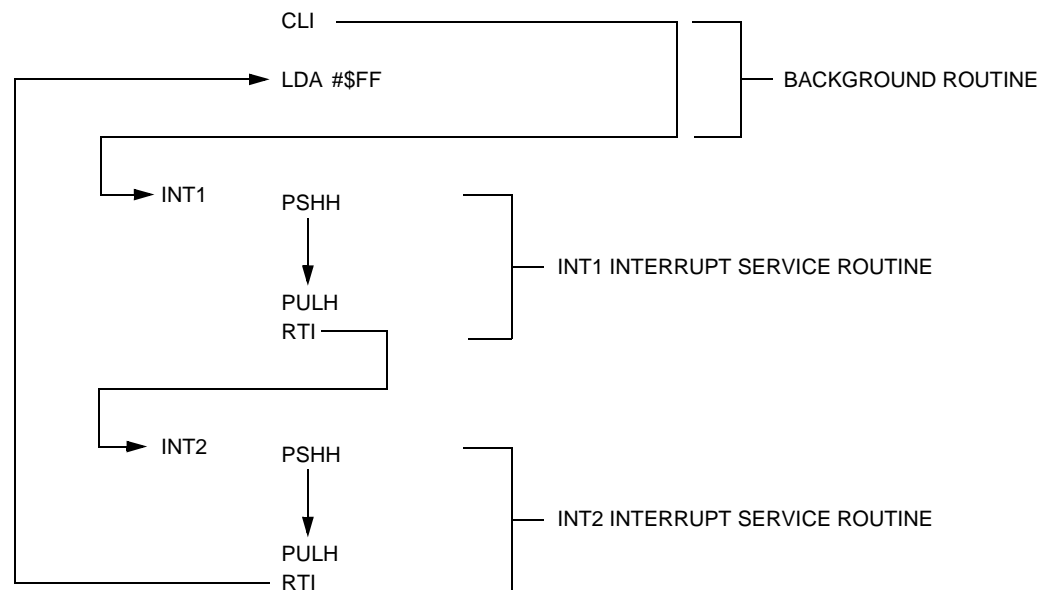
Figure 8-9. Interrupt Recognition Example
