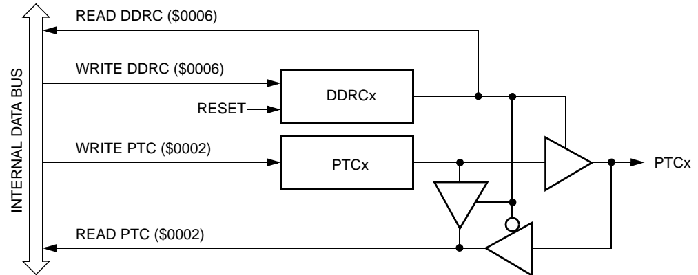
Figure 20-9. Port C I/O Circuit
