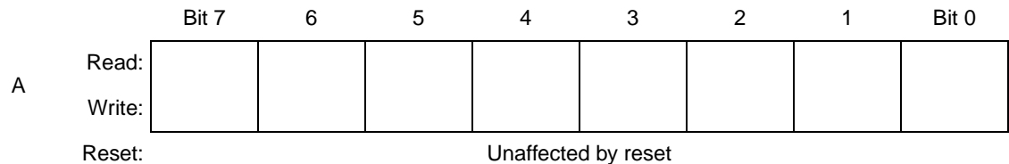
Figure 7-2. Accumulator (A)
