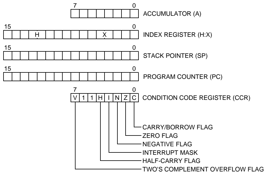
Figure 7-1. CPU Registers
