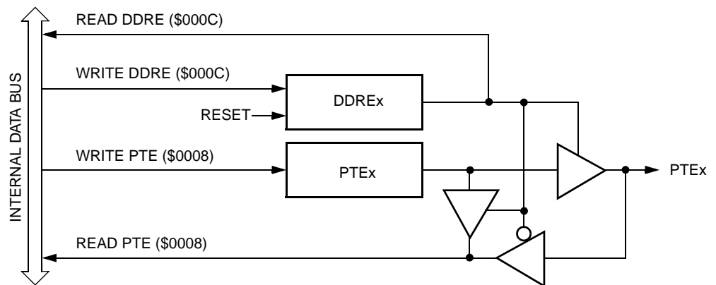
Figure 20-15. Port E I/O Circuit
