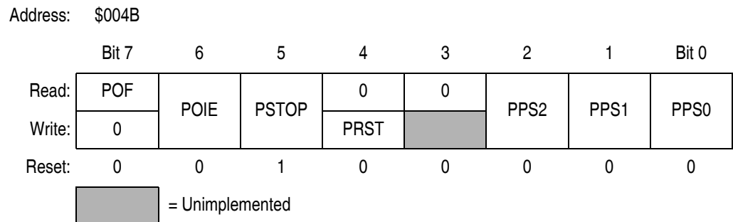
Figure 19-3. PIT Status and Control Register (PSC)
