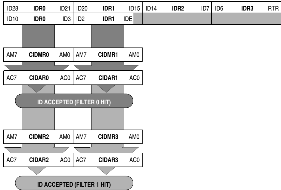
Figure 21-4. Dual 16-Bit Maskable Acceptance Filters
