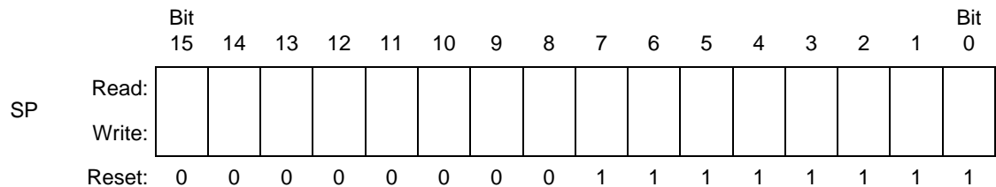
Figure 7-4. Stack Pointer (SP)
