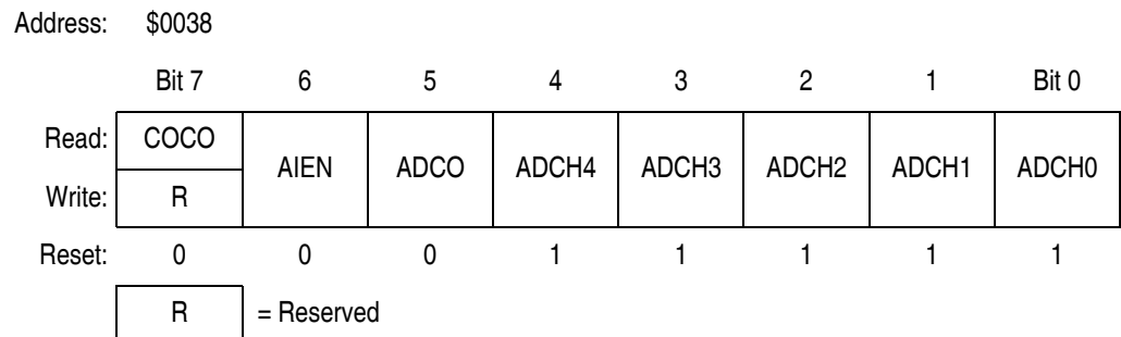
Figure 24-2. ADC Status and Control Register (ADSCR)
