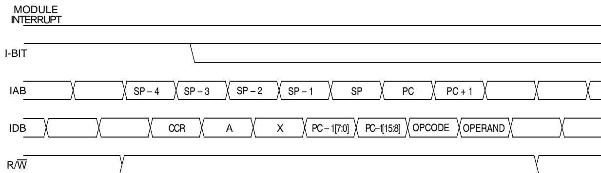
Figure 8-8. Interrupt Recovery
