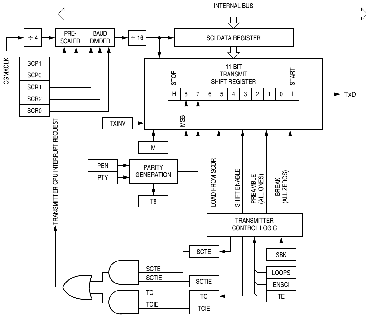
Figure 16-4. SCI Transmitter
