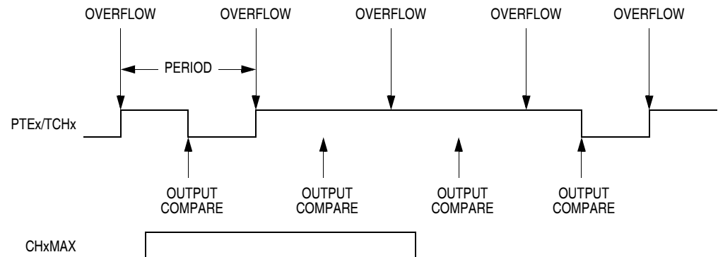
Figure 18-8. CHxMAX Latency
