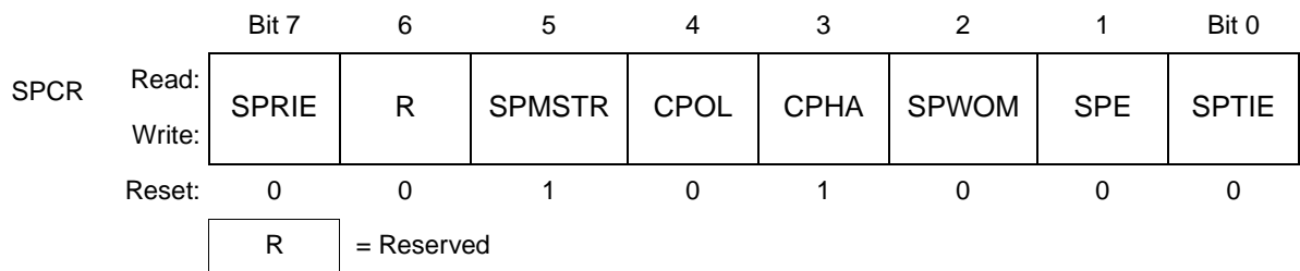
Figure 17-12. SPI Control Register (SPCR)
