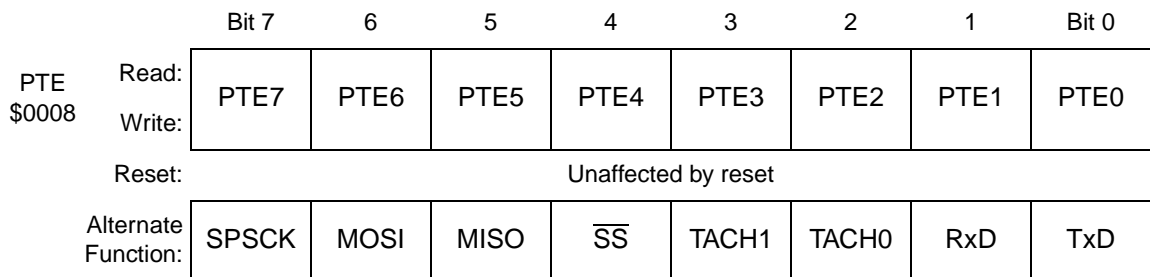
Figure 20-13. Port E Data Register (PTE)
