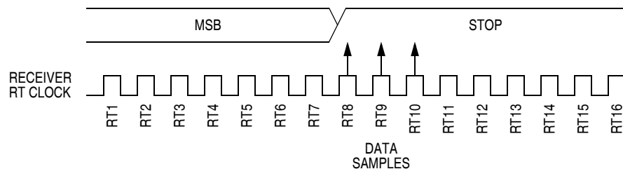
Figure 16-9. Slow Data
