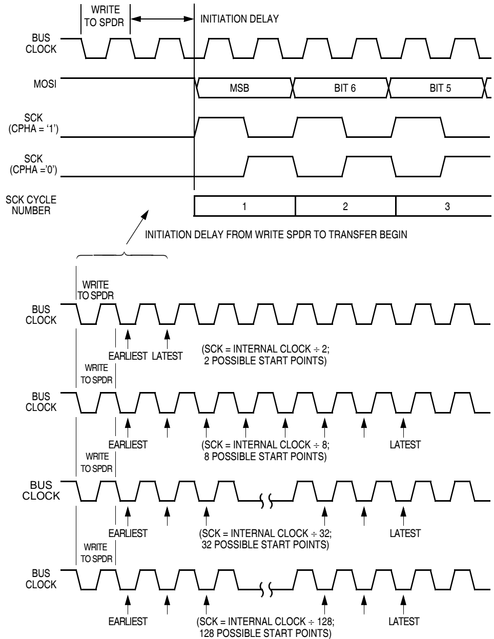
Figure 17-6. Transmission Start Delay (Master)
