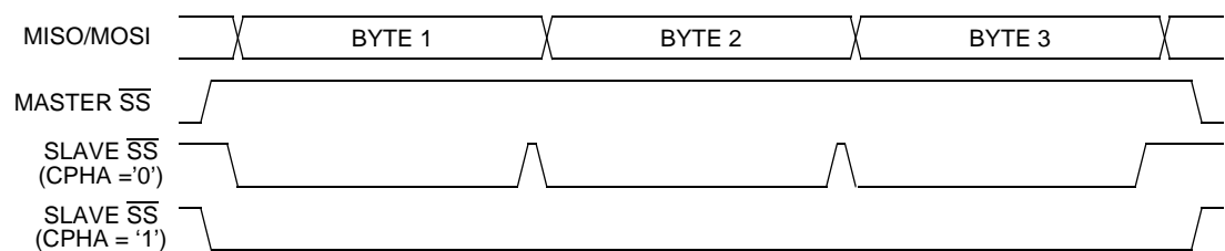
Figure 17-11. CPHA/ \overline{SS} Timing
