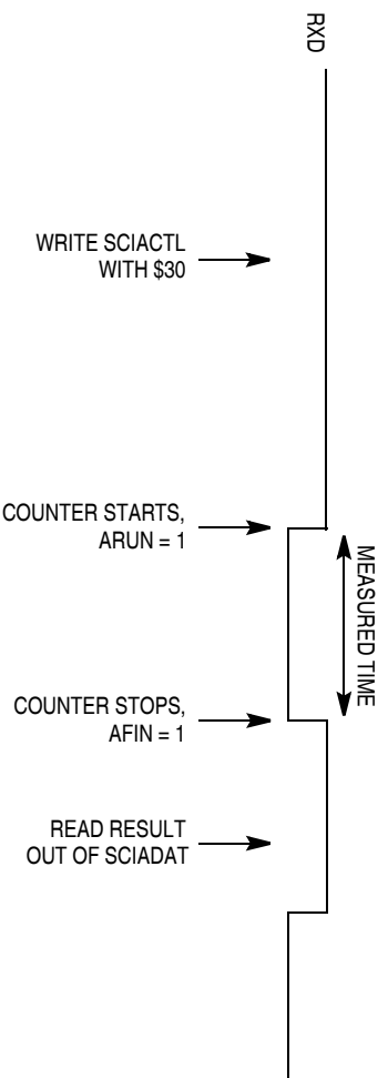
Figure 13-22. Bit Time Measurement with ACLK = 1, Scenario B
