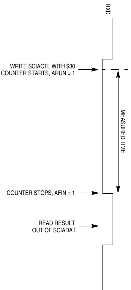
Figure 13-21. Bit Time Measurement with ACLK = 1, Scenario A
