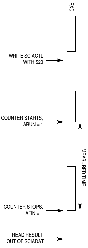
Figure 13-20. Bit Time Measurement with ACLK = 0
