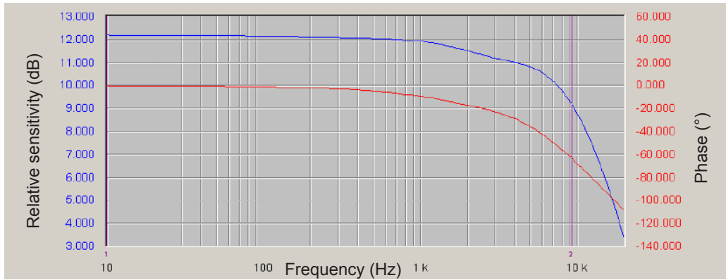
Figure 1: Frequency response
