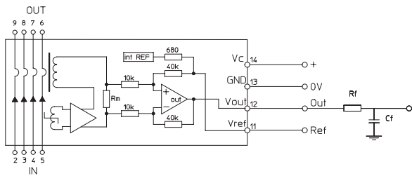
Figure 31: Test connection
