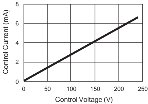
Figure 2c — DRL48A35 relay
