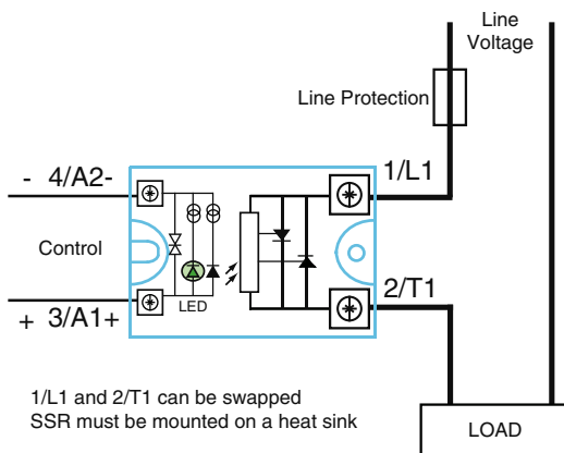
Figure 1b — STH relays, 35A and above
