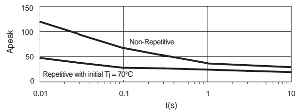
Figure 5a — X24D12 relay
