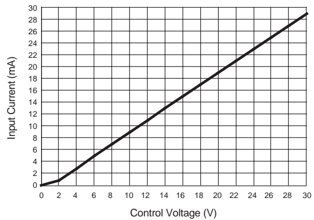
Figure 4 — X relays
