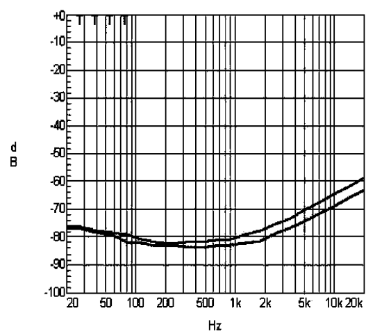
Figure 19 PSRR vs. Freq SE mode, 3V, 320Ohm, 200mVpp Input terminated
