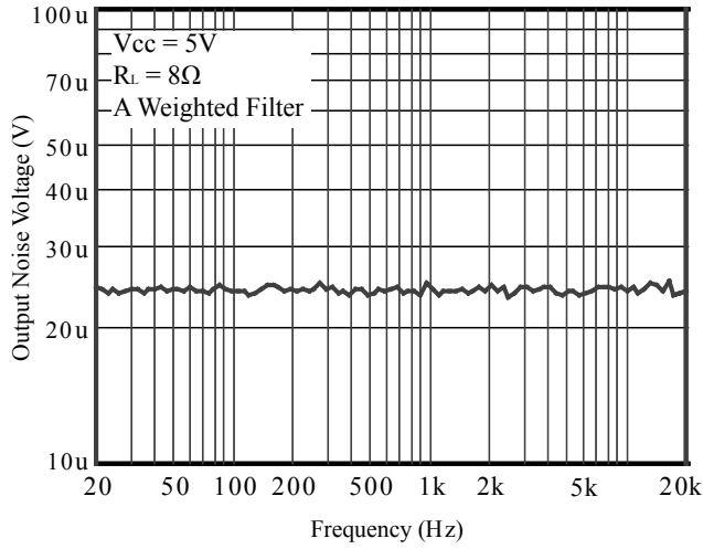
Figure 9 Noise Floor
