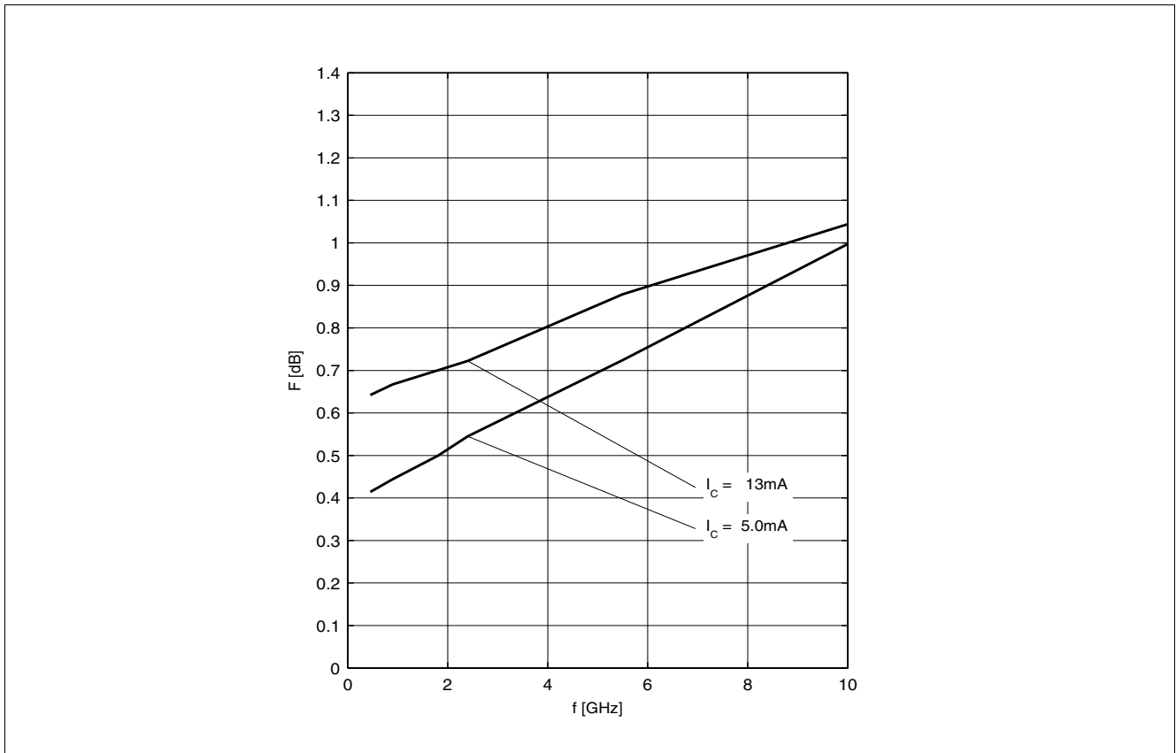
Figure 13 Noise Figure NF_{\min} = f(\text{freq}) , V_{CE} = 3\text{ V} , Z_S = Z_{\text{opt}}
