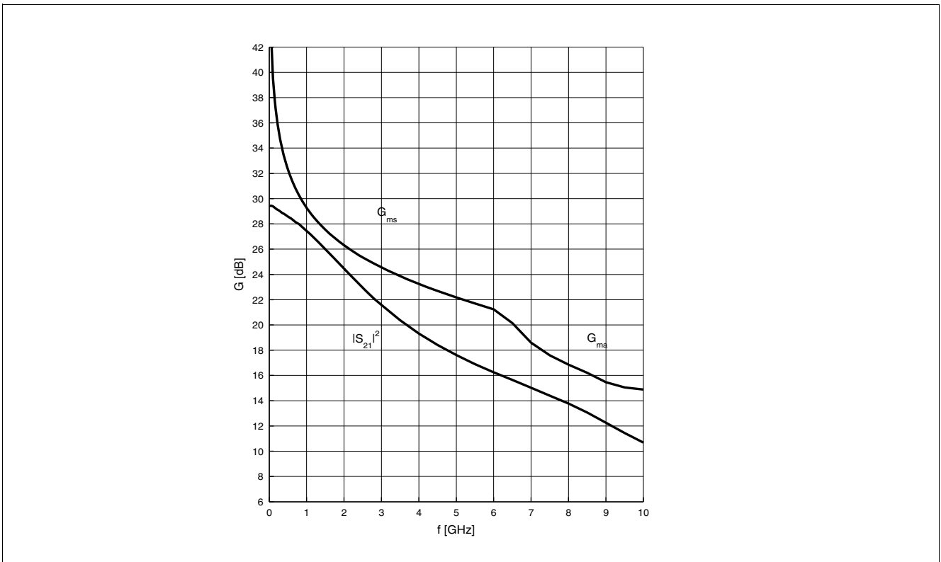
Figure 6 Power Gain G_{ma} , G_{ms} , |S_{21}|^2 = f(\text{freq}) , V_{CE} = 3 \text{ V} , I_C = 13 \text{ mA}
