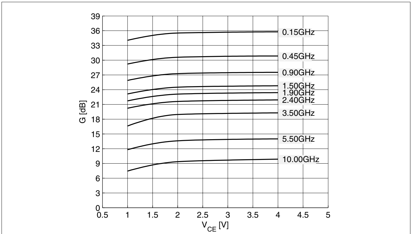
Figure 13 Maximum Power Gain G_{max} = f(V_{CE}) , I_C = 60\text{ mA} , f = \text{Parameter in GHz}
