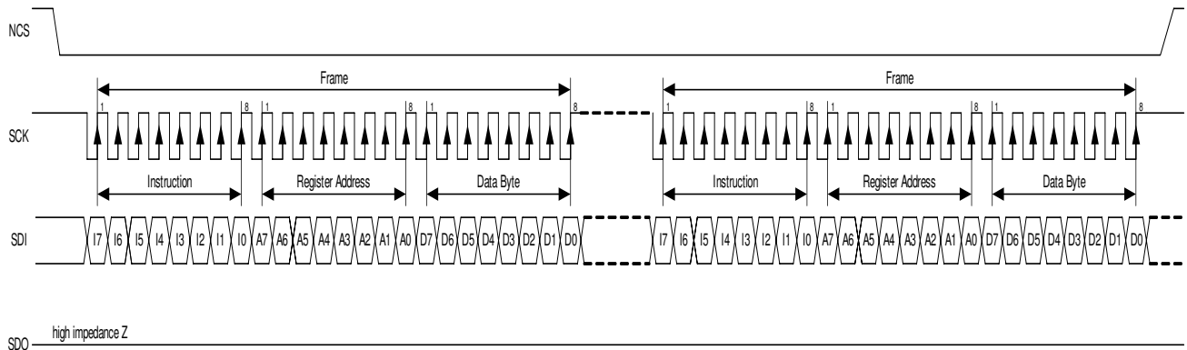
Figure 61 Write Register
