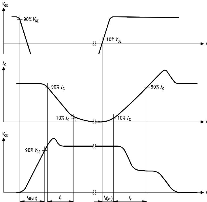
Figure A. Definition of switching times
