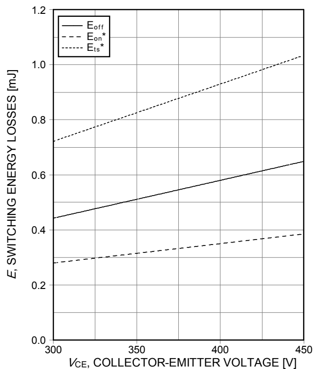
Figure 16. Typical switching energy losses as a function of collector emitter voltage (inductive load, T_{vj}=175^\circ\text{C} , V_{GE}=15/0\text{V} , I_C=10\text{A} , r_G=23\Omega , Dynamic test circuit in Figure E)
