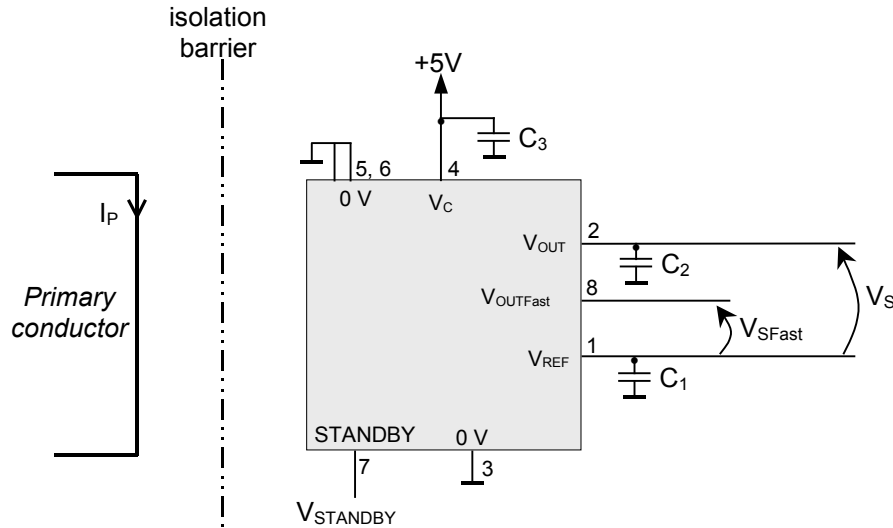
Figure 6: Typical connection diagram ( C_1 = C_3 = 47 \text{ nF} , C_2 = 4.7 \text{ nF} )
