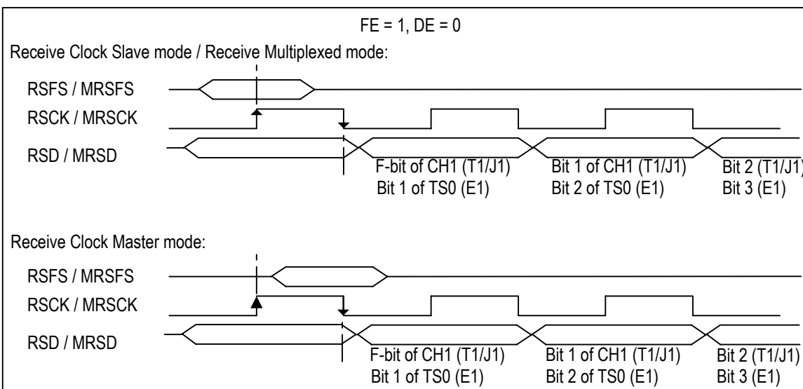
Figure 24. No Offset When FE = 1 & DE = 0 In Receive Path
