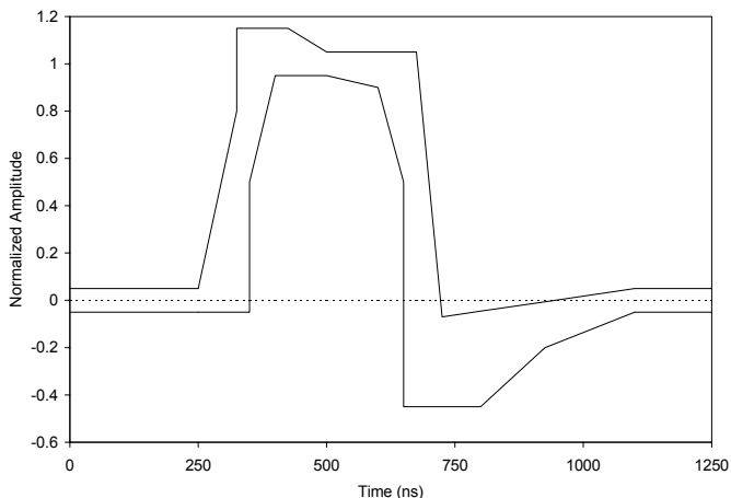
Figure 32. DSX-1 Waveform Template
