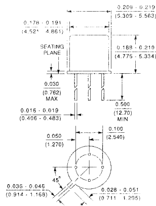
Package Dimensions TO-72
