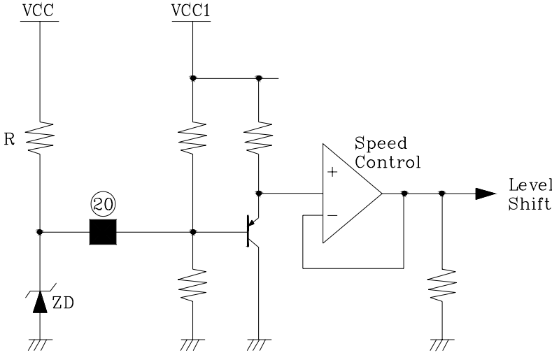
Fig6. Thy motor speed control
