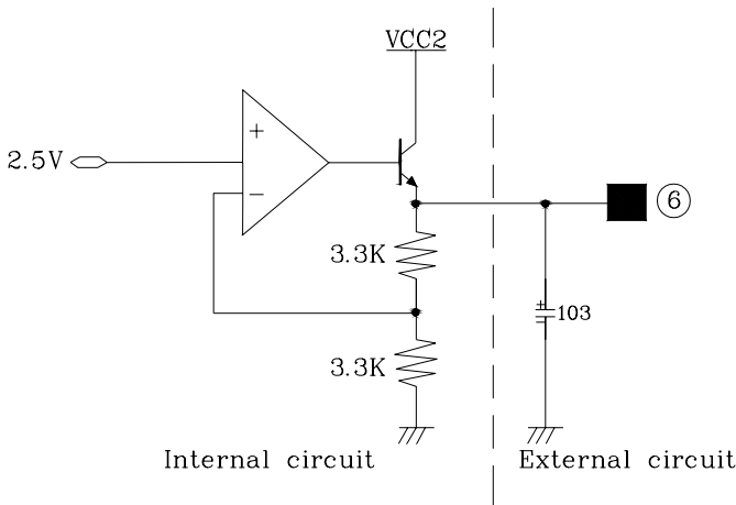
Fig7. Regulator
