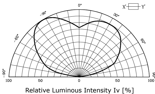
Fig. 5-2 Radiation Diagram(Y)
