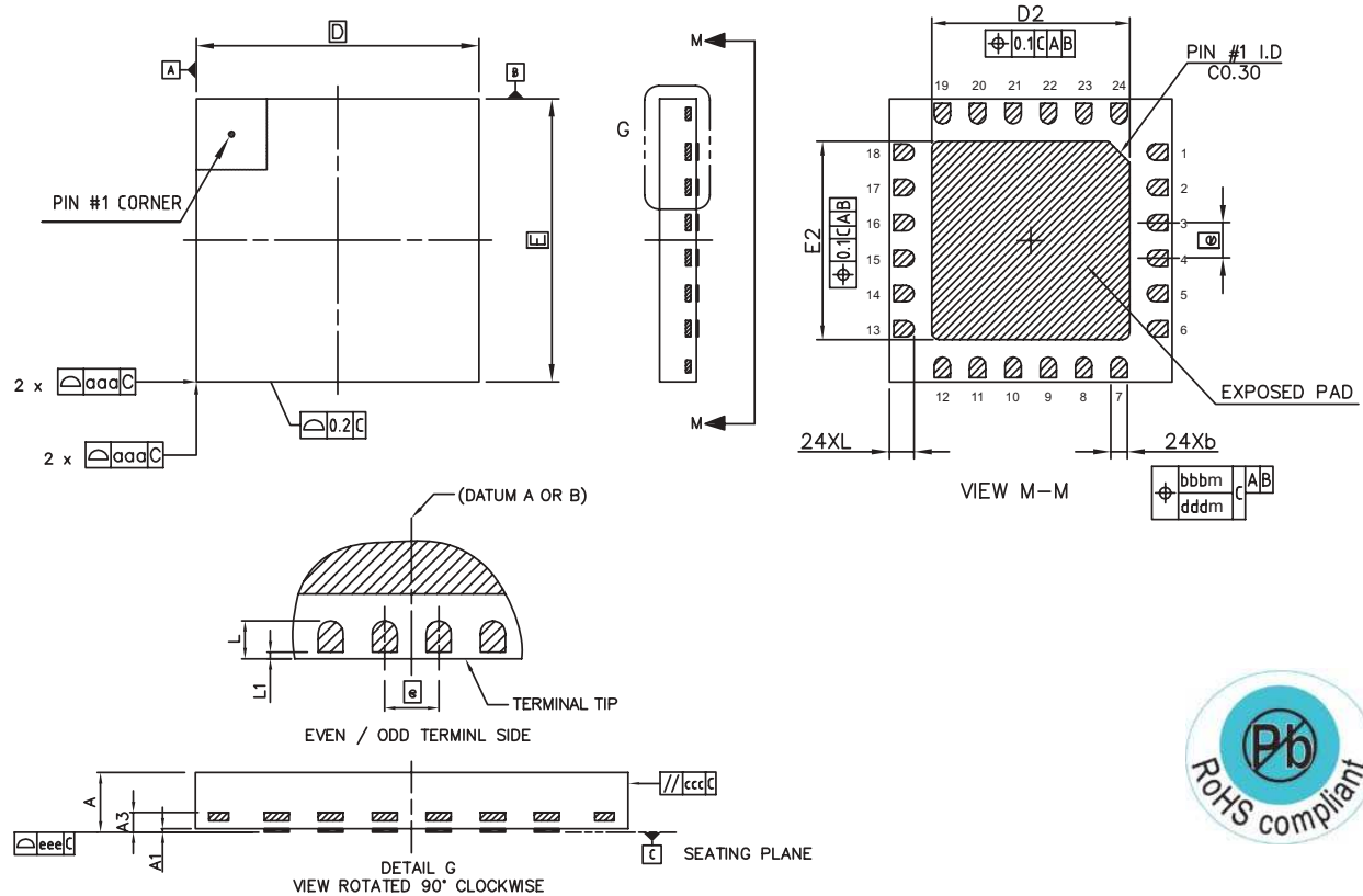
Figure 21. TQFN(4x4)-24 Package
