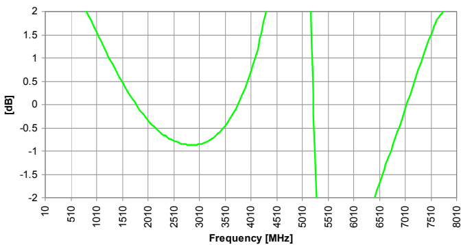
Amplitude Balance
