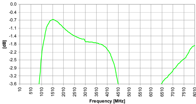
Insertion Loss
