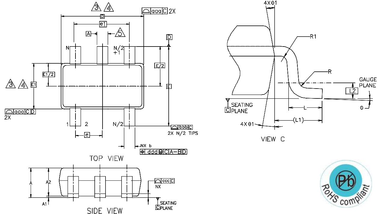
Figure 22. TSOT23-5 Package
