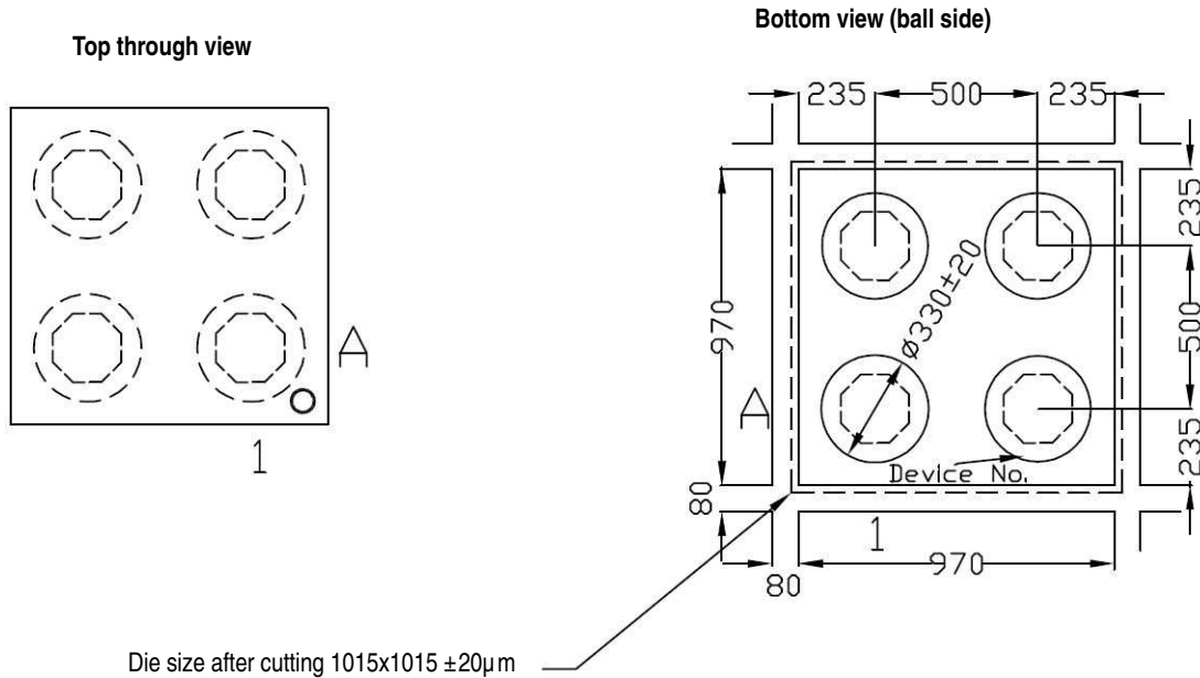
Figure 50. 4-bump WL-CSP Package
