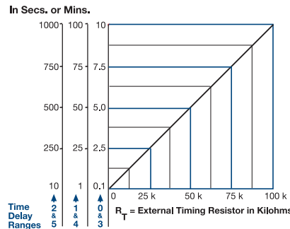
This chart applies to externally adjustable part numbers. The time delay is adjustable over the time delay range selected by varying the resistance across the R_T terminals; as the resistance increases the time delay increases. When selecting an external R_T , add the tolerances of the timer and the R_T for the full time range adjustment. Examples: 1 to 50 S adjustable time delay, select time delay range 1 and a 50 K ohm R_T . For 1 to 100 S use a 100 K ohm R_T .
