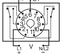
11-pin DPDT
