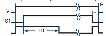
Delay-on-Make (Normally Closed)
