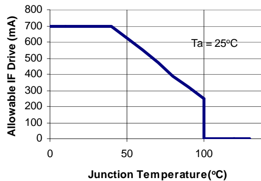
Derating Curve
