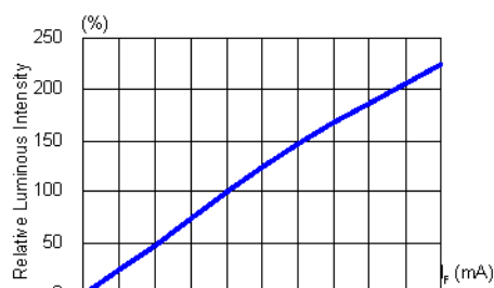
Fig.2 Luminous Intensity vs. Forward Current
