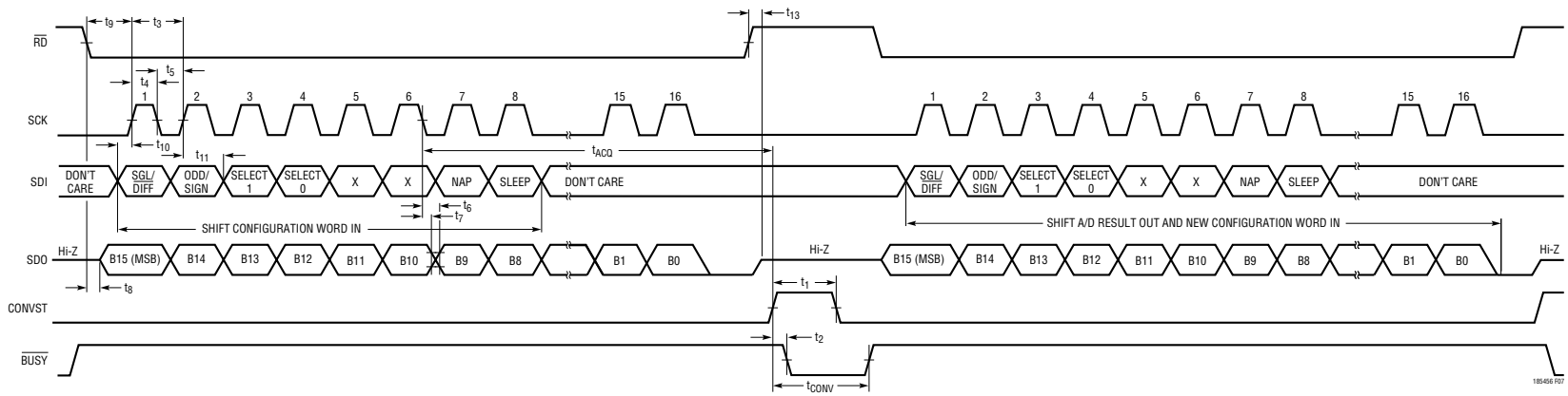
Figure 7. Operating Sequence for the LTC1856*
