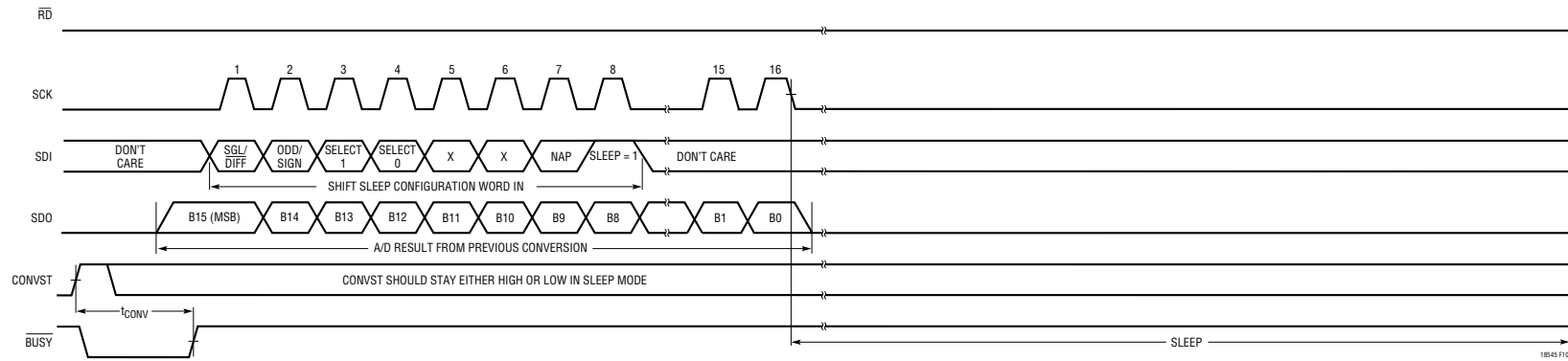
Figure 10. Sleep Mode Operation for the LTC1856*
