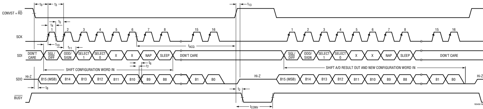
Figure 6b. Mode 2 for the LTC1856*. CONVST and \overline{RD} Tied Together. CONVST Starts a Conversion, Data is Read by \overline{RD}
