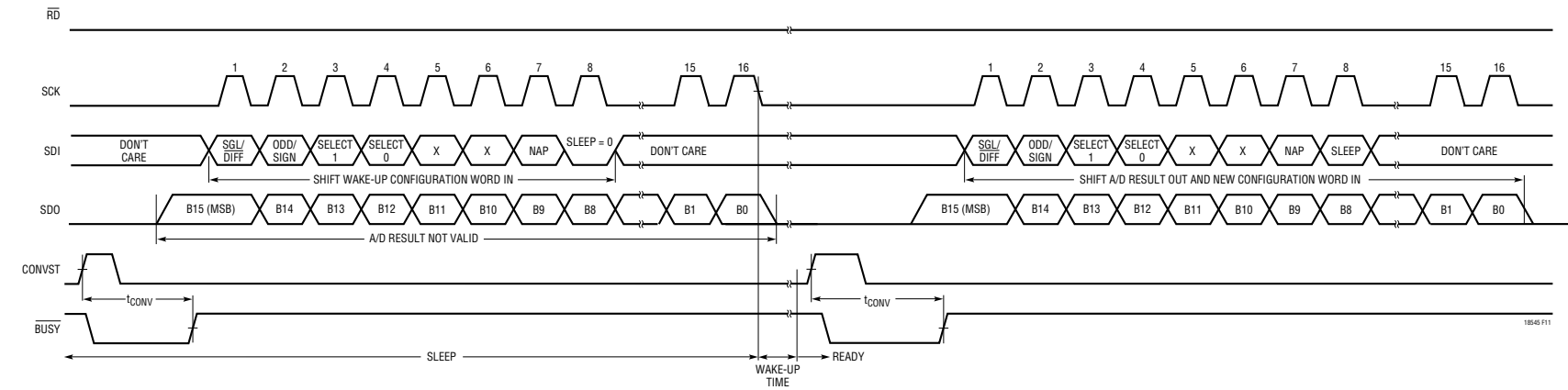
Figure 11. Wake Up from Sleep Mode for the LTC1856*
