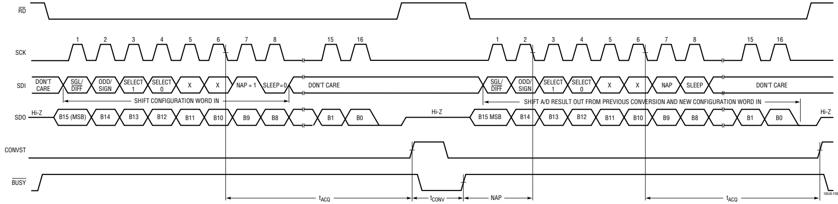
Figure 9. Nap Mode Operation for the LTC1856*
