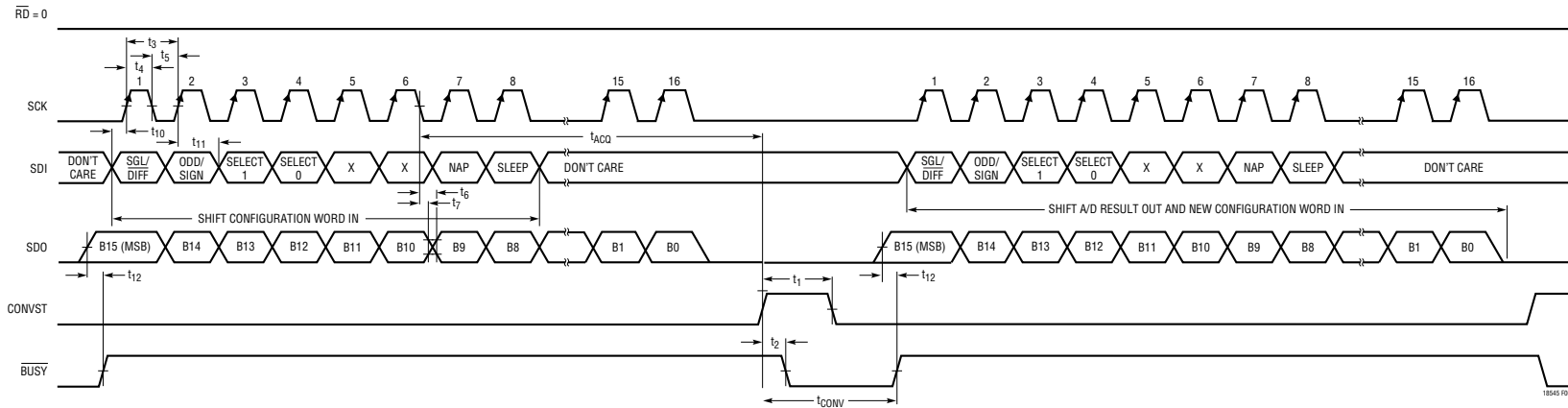
Figure 6a. Mode 1 for the LTC1856*. CONVST Starts a Conversion, Data Output is Always Enabled ( \overline{RD} = 0 )
