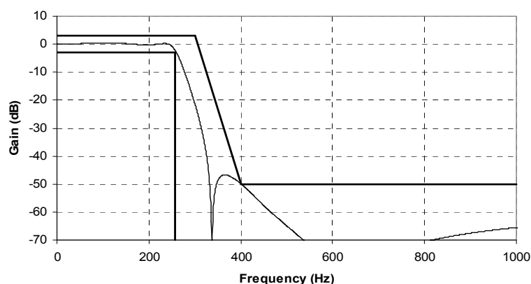
Figure 17 Low Pass Sub-Audio Band Filter for CTCSS and DCS
