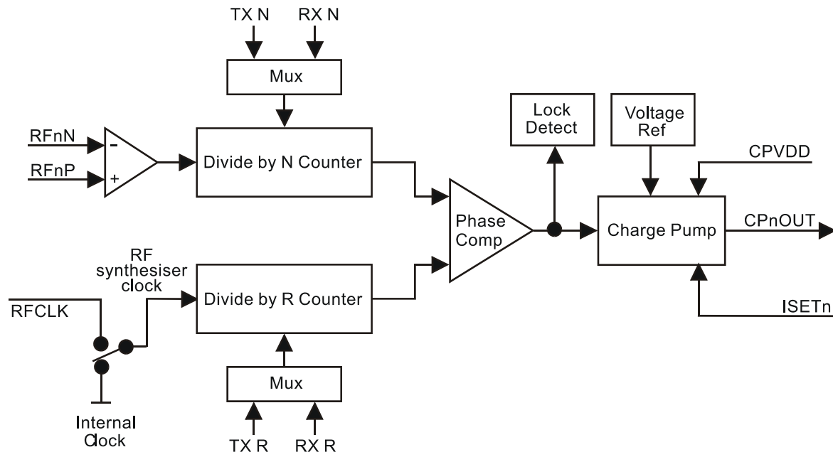
Figure 23 Single RF Channel Block Diagram
