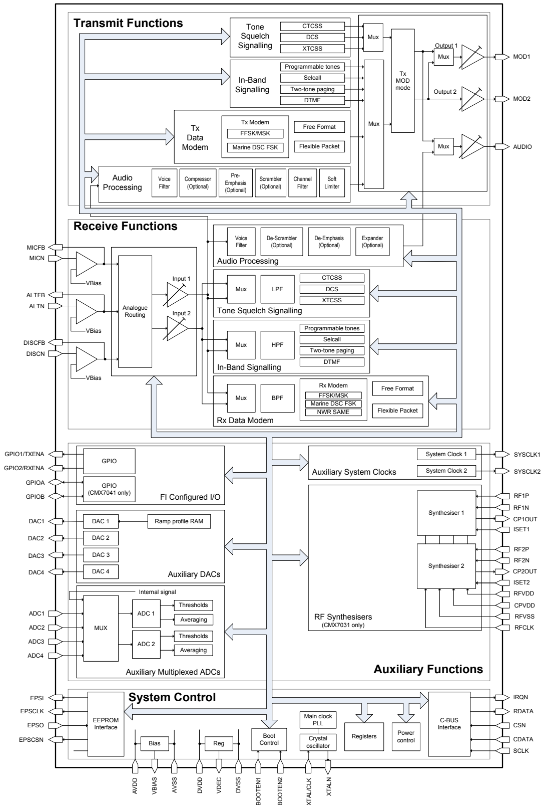
Figure 1 Block Diagram
