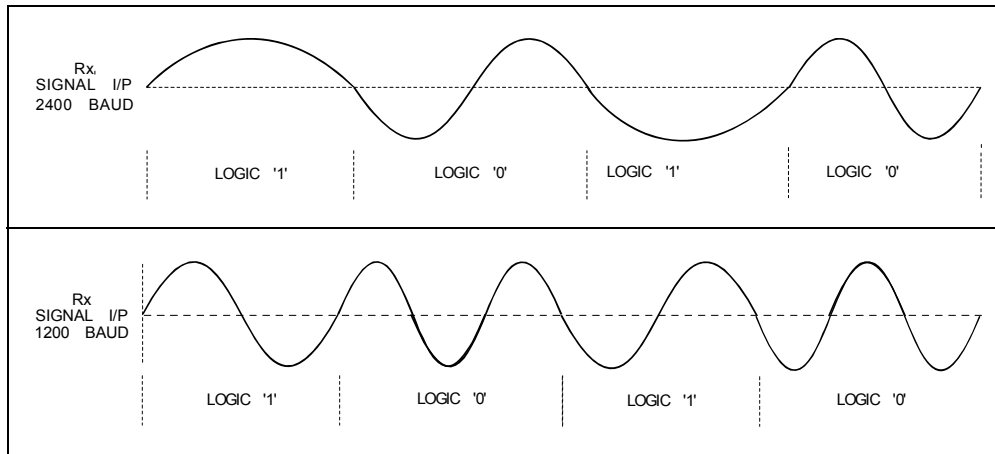
Figure 18 Modulating Waveforms for 1200 and 2400 Baud MSK/FFSK Signals
