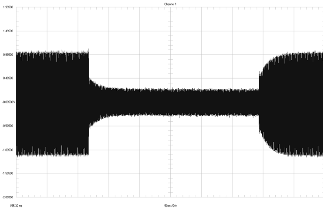
Figure 15 Expandor Transient Response
