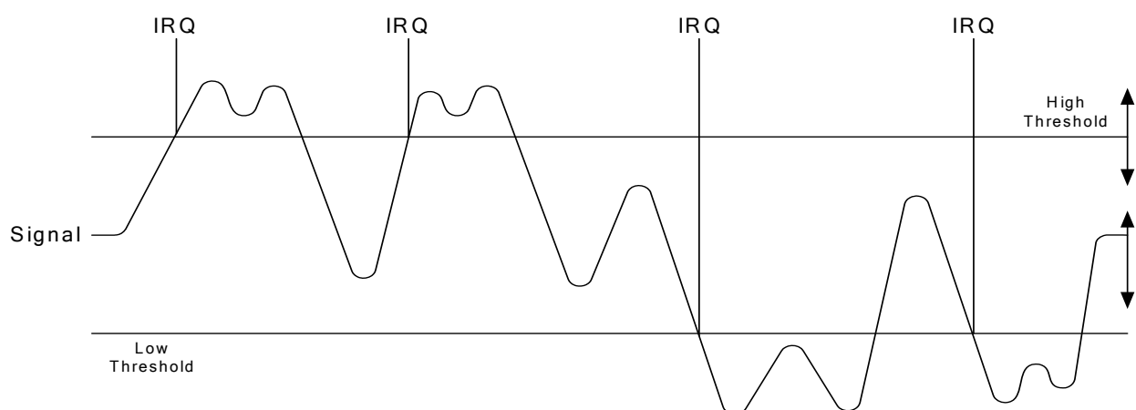
Figure 21 AuxADC IRQ operation
