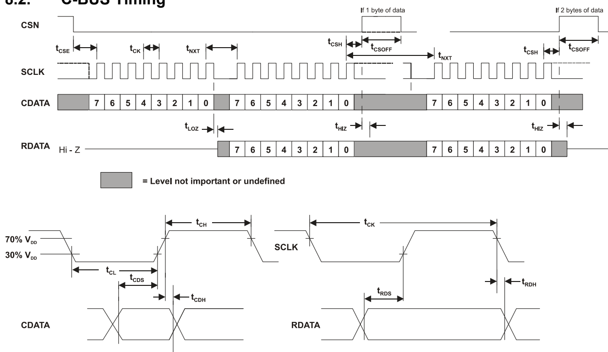
Figure 26 C-BUS Timing
