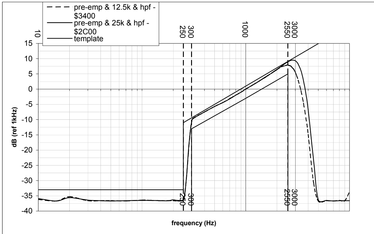
Figure 14 Audio Frequency Pre-emphasis
