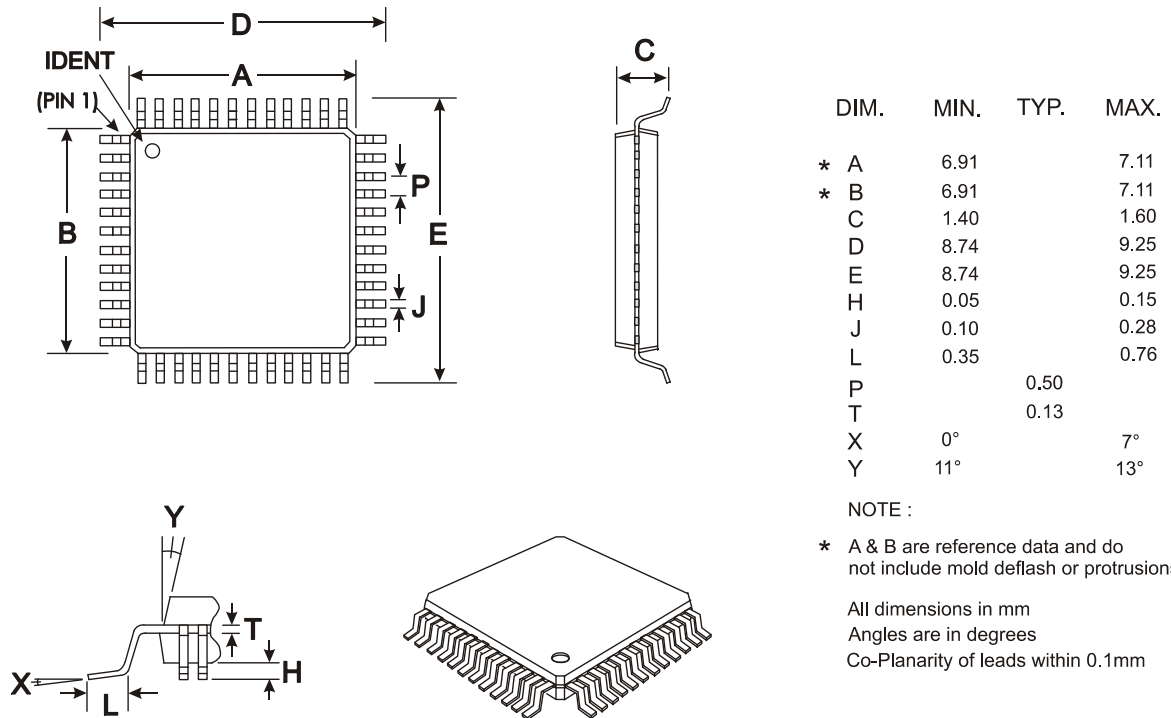
Figure 30 Mechanical Outline of 48-pin LQFP (L4)
