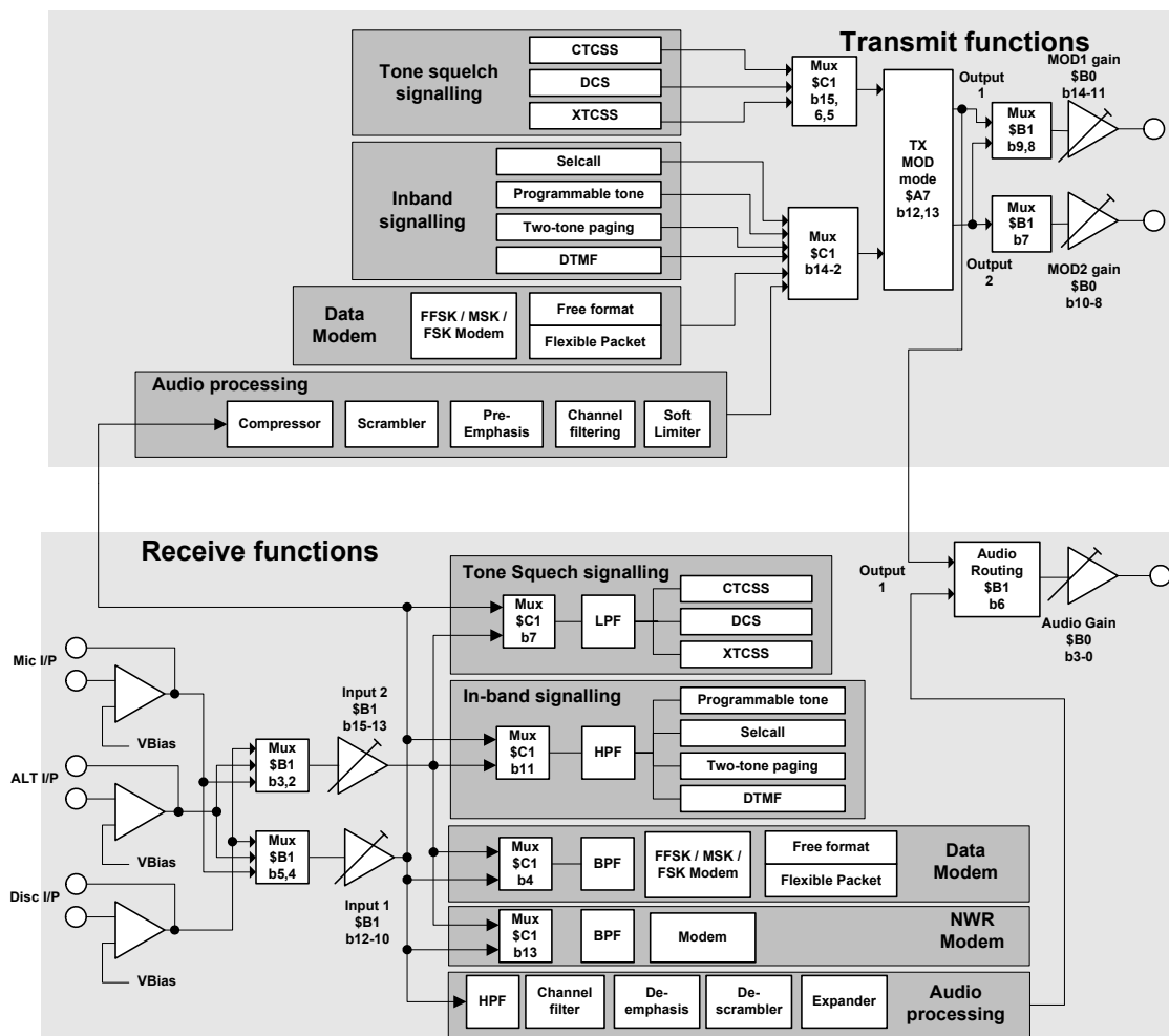
Figure 9 Signal Routing
