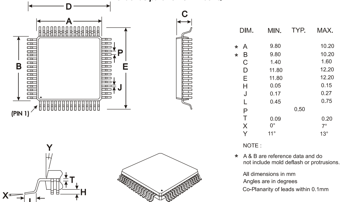
Figure 28 Mechanical Outline of 64-pin LQFP (L9)
