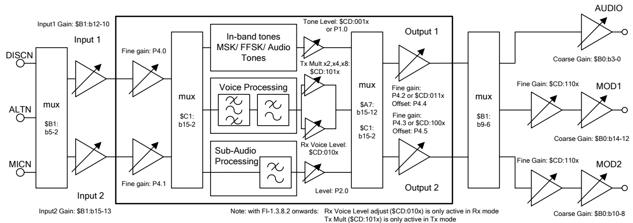
Figure 25 Level Adjustments
