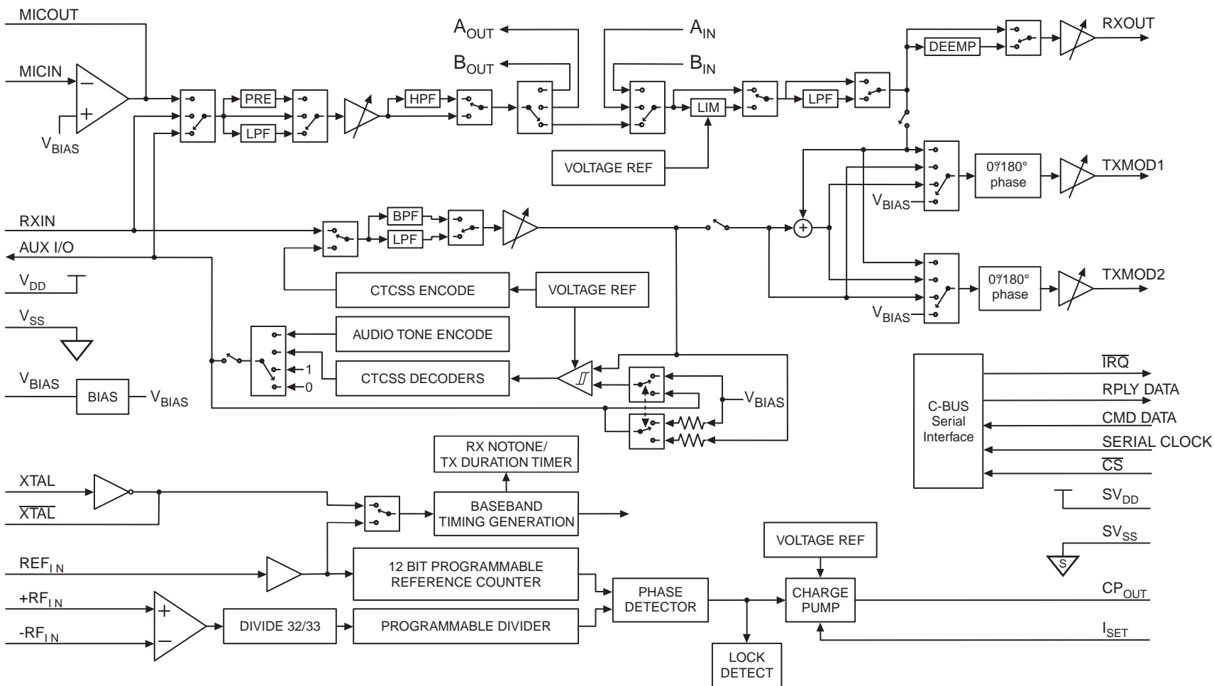
Figure 1: Block Diagram
