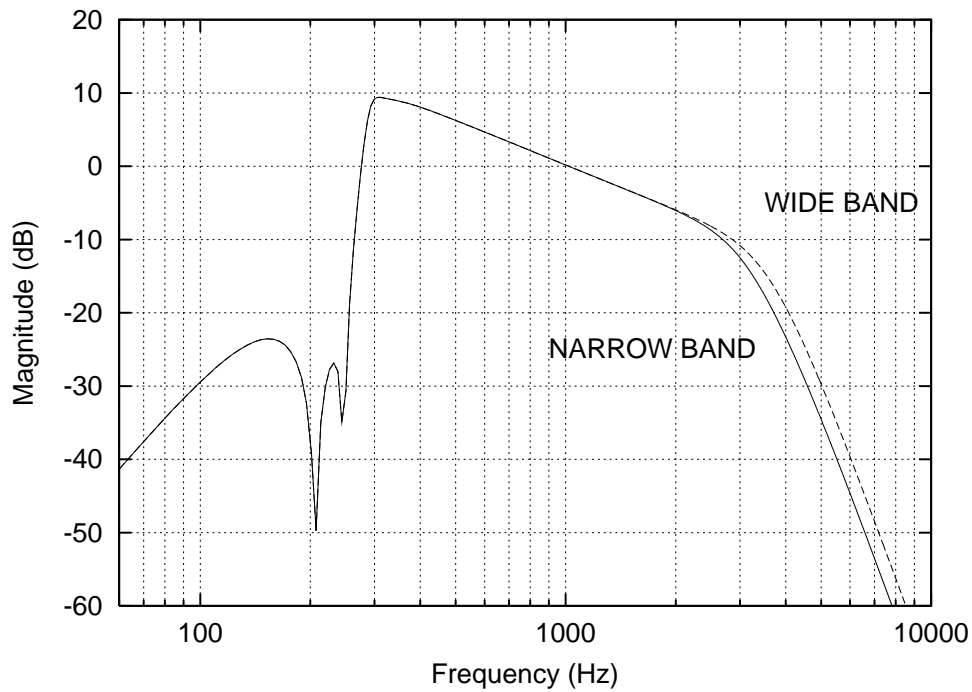
Figure 12: Receive audio path frequency response with de-emphasis.
