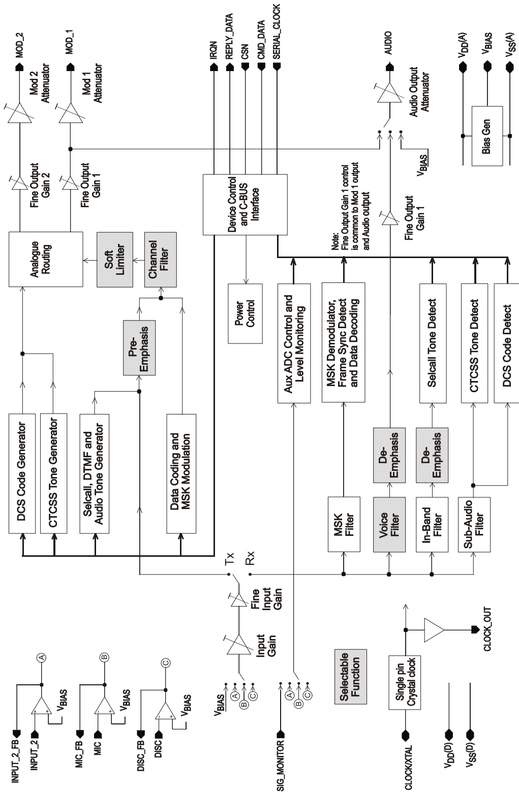
Figure 1 Block Diagram
